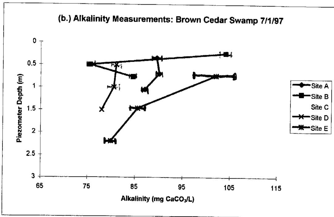
Figure 8: Alkalinity Measurements for Brown Cedar Swamp
