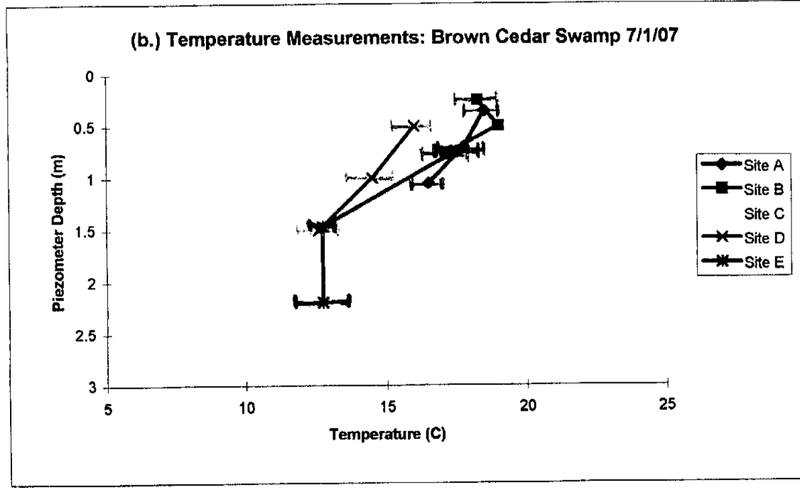
Figure 2: Temperature Variation at Brown Cedar Swamp Temperature trends are shown for Brown Cedar Swamp for the first and second sampling periods, in Figures a and b, respectively. Sites A-E represent the individual piezometer nests, with A being located closest to the stream. Error bars represent the standard deviation on the means for pipes of identical depth at each nest. Data clearly indicate that temperature decreases with depth for each sampling period.
