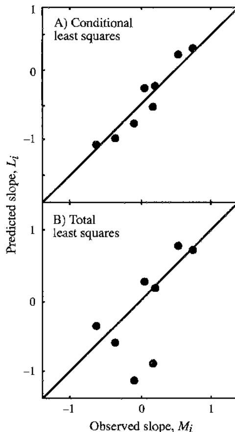
FIG. 4. The predicted change in average annual biomass with average annual planktivity for each species, L_i , vs. the observed change, M_i . (A) L_i was predicted using coefficients obtained from conditional least-squares estimation. (B) L_i was predicted using coefficients obtained from total least-squares estimation. Each point corresponds to a zooplankton species, although Chaoborus is excluded (see Results: Long-term changes).
