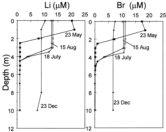
Figure 5. Depth profiles of the concentrations of \text{Li}^+ and \text{Br}^- in West Long Lake during 1992 (the first year of LiBr addition). Each line represents a profile taken on a different date (solid squares, 23 May; open circles, 18 July; solid triangles, 15 August; solid diamonds, 23 December). Autumnal mixing occurred in October.
