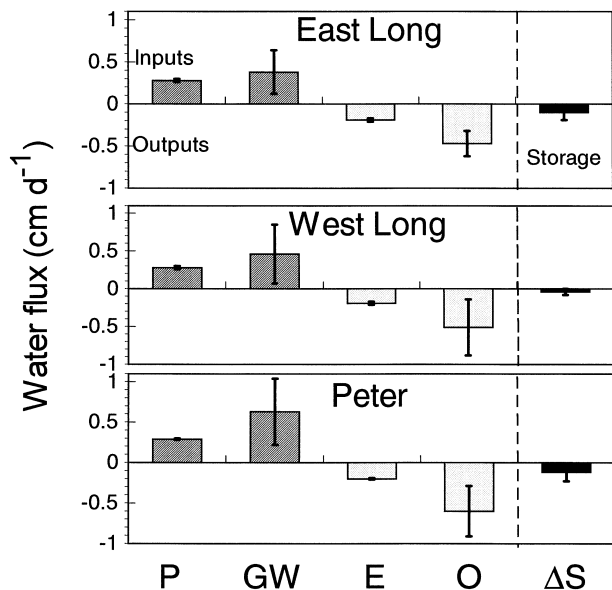
Figure 9. Average water budgets for the three lakes, based on the addition of LiBr. Shown are mean fluxes for the period of record (1992–96 in East and West Long Lakes and 1993–96 in Peter Lake) along with standard deviations representing interannual variation. P, precipitation input; GW, groundwater input; E, evaporation; O, outflowing water in seepage plus surface flow; ΔS, the change in water storage (volume) in the lake. Positive values are inputs and negative values are outputs. For ΔS, a loss in volume is plotted here as a negative value.
