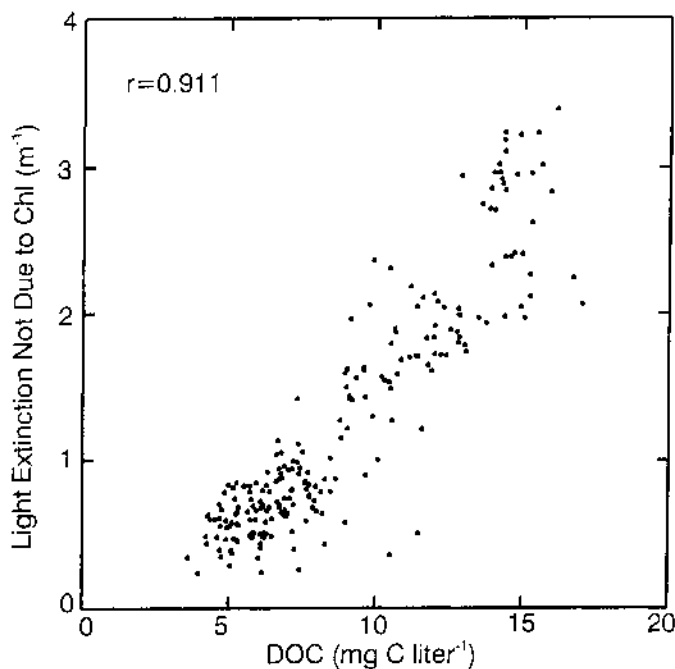
Fig. 8. Scatter plot of light extinction that is not explainable by chlorophyll vs. DOC concentration ( n = 219 ).
