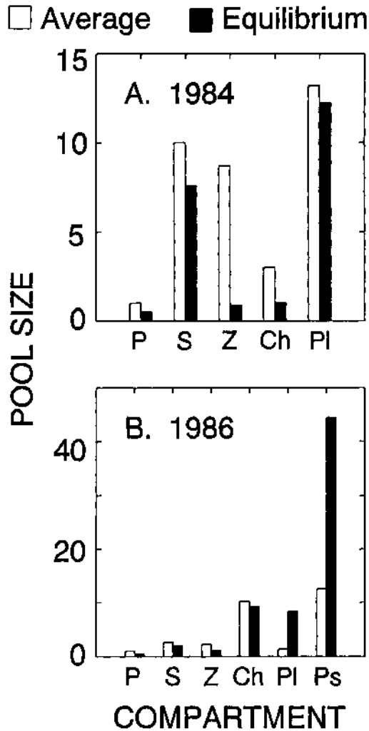
FIG. 3.—Equilibrium and summer average phosphorus pool sizes ( \mu\text{g L}^{-1} ) in Tuesday Lake for summers of (A) 1984 and (B) 1986. Compartments: P, dissolved P; S, seston; Z, zooplankton; Ch, Chaoborus ; Pl, planktivorous fish; Ps, piscivorous fish.
