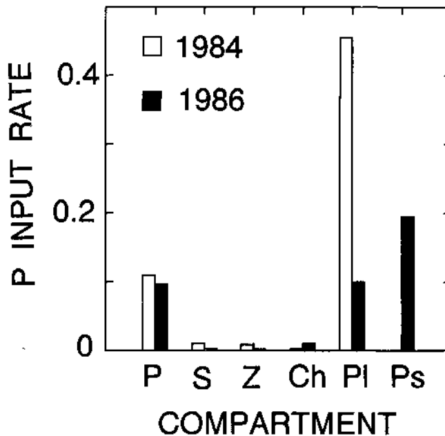
FIG. 2.—Phosphorus input rate ( \mu\text{g L}^{-1} \text{d}^{-1} ) to Tuesday Lake during June–August of 1984 and 1986 from sources described in the text. Compartments: P, dissolved P; S, seston; Z, zooplankton; Ch, Chaoborus ; Pl, planktivorous fish; Ps, piscivorous fish.
