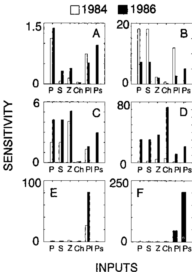
FIG. 4.—Sensitivities ( dx^*/dz_i ) of phosphorus pool sizes to changes in phosphorus inputs for Tuesday Lake in the summers of 1984 and 1986. Each panel shows the sensitivity of one pool to changes in input rates to all pools. A, dissolved P; B, seston; C, zooplankton; D, Chaoborus ; E, planktivores; F, piscivores. Inputs: P, dissolved P; S, seston; Z, zooplankton; Ch, Chaoborus ; Pl, planktivorous fish; Ps, piscivorous fish.
