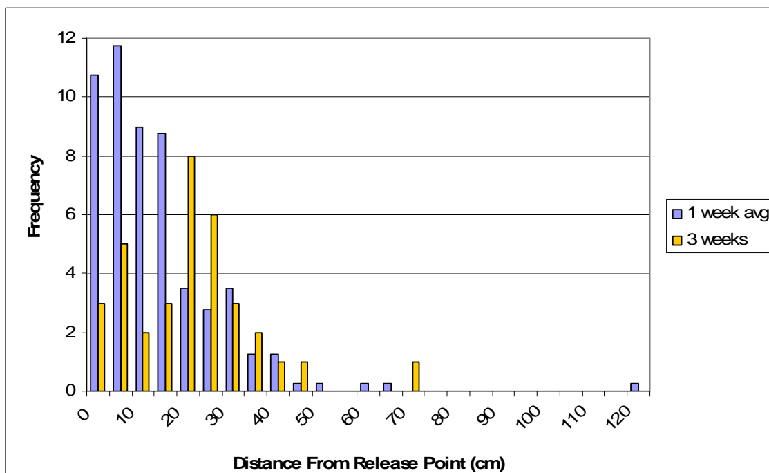
Figure 6. Histogram for plots without leaves at one week and three week time points for tagged Aporrectodea spp.. The one week values are an average of the frequencies (N=4) of treated plots at each distance. The three week time point is the total reported treated distribution (N=1).
