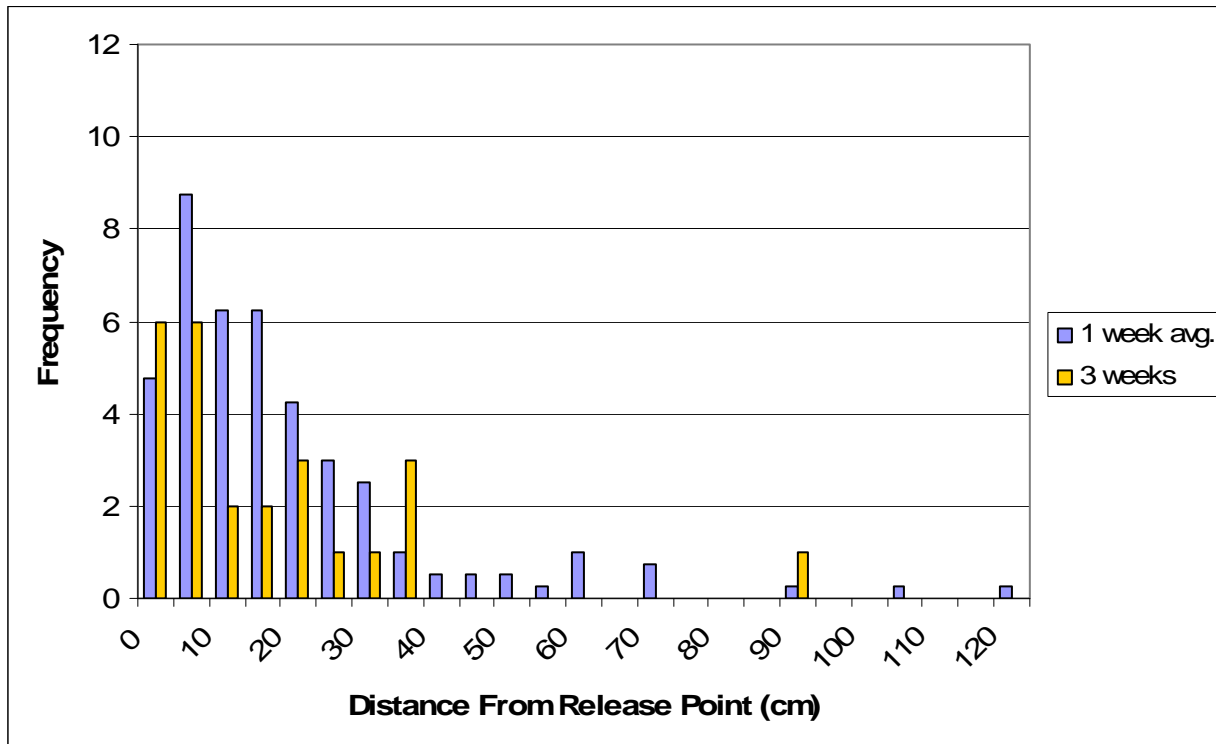
Figure 7. Histogram for plots with leaves at one week and three week time points for tagged Aporrectodea spp.. The one week values are an average of the frequencies (N=4) of treated plots at each distance. The three week time point is the total reported treated distribution (N=1).
