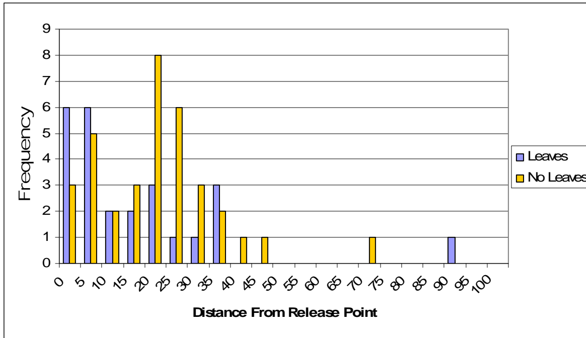
Figure 5. Histogram of the frequency of distance moved by tagged Aporrectodea spp. at three week time point.
