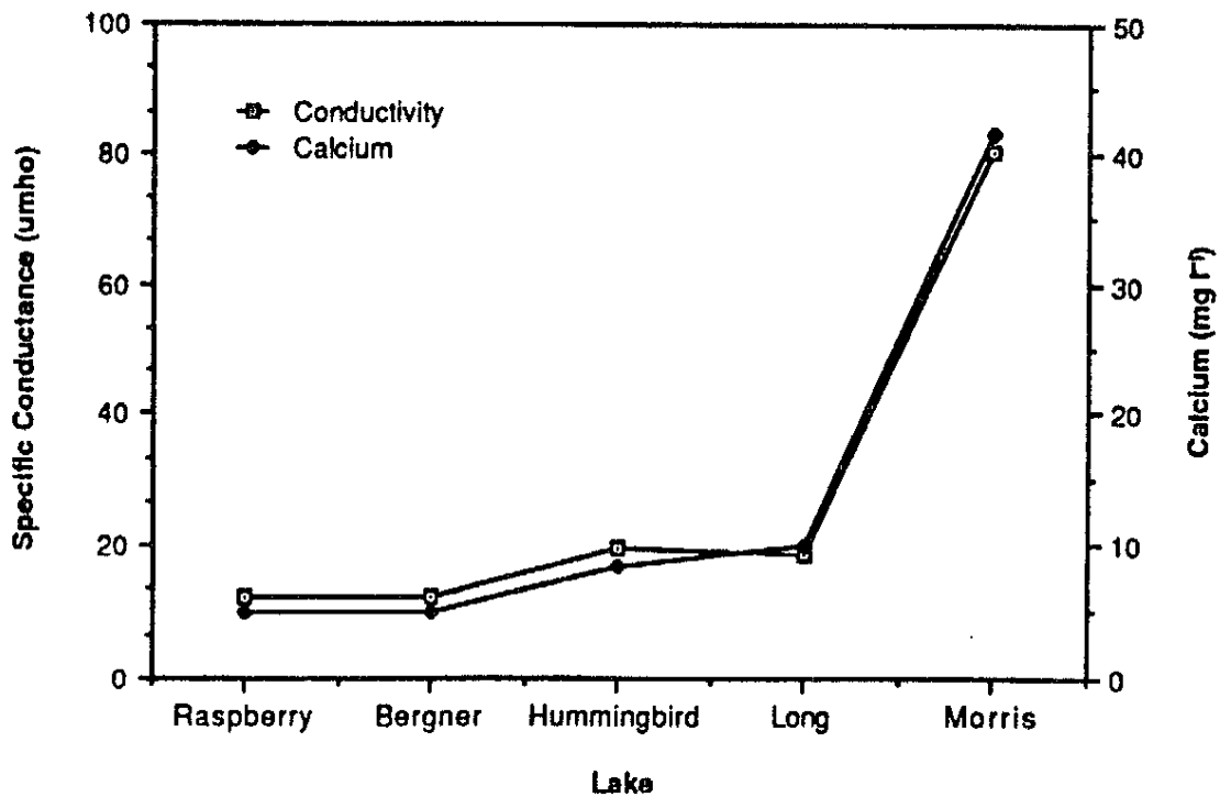
Fig.5 Specific conductance of the lakewater as an indicator of calcium content.
