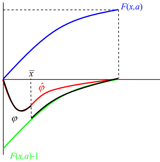
Figure A.2: An example of a discontinuous co-state function due to a violation of (19) when \bar{x} < \tilde{x} = 1 .
