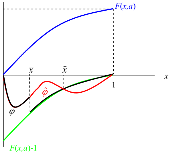
Figure A.1: An example of a discontinuous co-state function due to a violation of (19) when \bar{x} < \tilde{x} < 1
