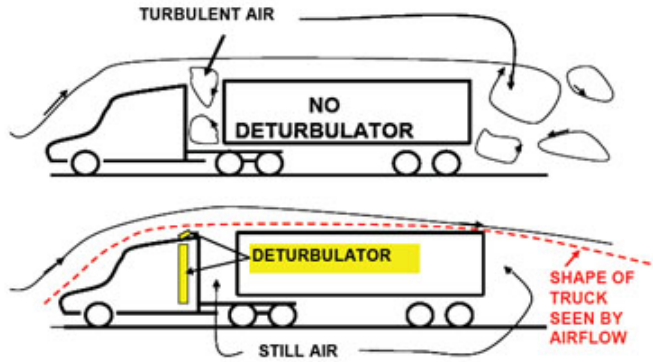
Figure 11 – Effect of deturbulator on a tractor trailer [95]
