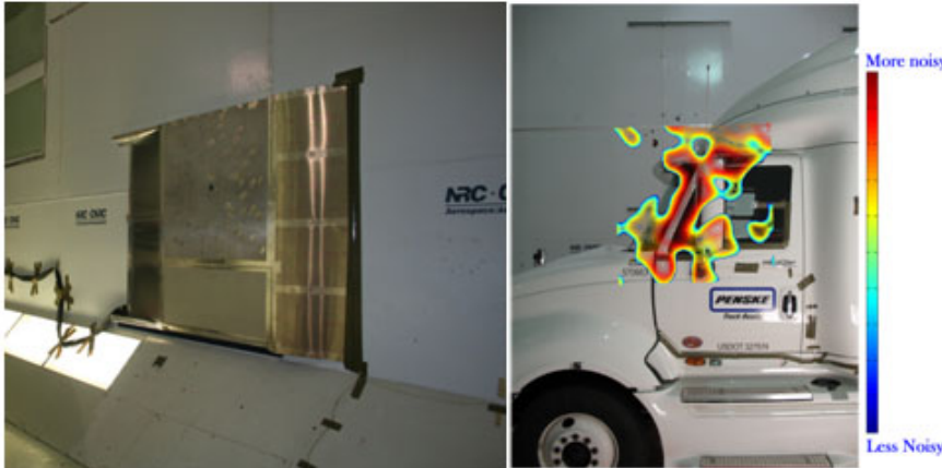
Figure 30 – NRC aero-acoustic array mounted to side-wall of 9 m x 9 m Wind Tunnel (left) and subset of preliminary acoustic measurements for a tractor (right).
