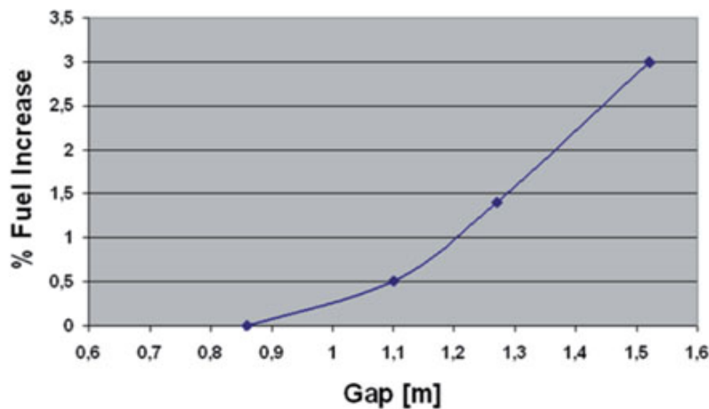
Figure 14 – Fuel burn increase vs. gap [99]
