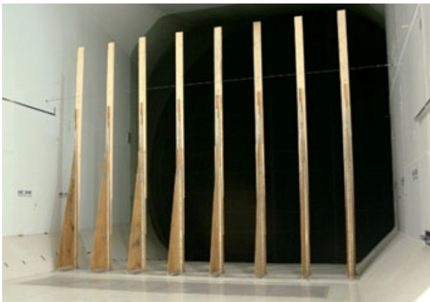
Figure 29 – Partial-height turbulence grid in NRC 9 m x 9 m Wind Tunnel
