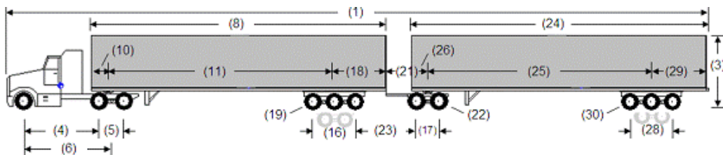
Figure 1 - Illustration of a long combination vehicle (LCV) [16]
