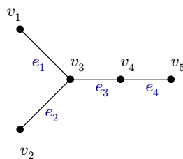
Figure 6.1: A tree T
