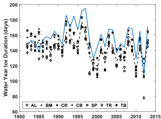
FIGURE 4. Lake ice duration from WYs 1982–2013. Dashed black line represents the mean value for all seven of the NTL-LTER lakes and bogs. OBS durations for individual lakes are represented with various symbols (see Table 1 for lake name abbreviations). Simulated values for a single lake (blue) using the VIC lake model with parameterization in Table E.2 of the Supporting Information Appendix E.
