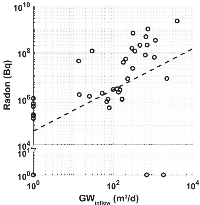
FIGURE 7. OBS radon measurements compared to average SIM daily inflowing GW discharges over WYs 2014–2015 for the 40 lakes surveyed across the NHLD during open water periods of 2015 and 2016. Near zero values for radon measurements and SIM inflowing GW discharges were set to a value of 1.0 in order to display low-end performance of the model (radon only, n = 2 ; SIM inflowing GW only, n = 6 ; both, n = 2 ). The dashed black line represents log-log linear regression best-fit line. Bq, Becquerel.
