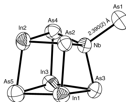
Figure 1. Structure of the cubane with a “handle” [\{\text{As}(\text{InAs}_3)\text{Nb}=\text{As}]^{7-} (ORTEP drawing; thermal ellipsoids at the 95% probability level). The unusually short distance of the handle is shown. The remaining distances [Å] are: Nb-As2 2.484(2), Nb-As3 2.526(2), Nb-As4 2.535(2), In1-As2 2.834(2), In1-As3 2.794(2), In1-As5 2.908(2), In2-As2 2.864(2), In2-As4 2.789(2), In2-As5 2.894(2), In3-As3 2.845(2), In3-As4 2.822(2), In3-As5 2.858(2). The angles [°] at Nb and As5 are in the range 107.26(7)–112.82(7) and 79.32(5)–80.27(5), respectively. The angles around As2, As3, and As4 fall in the range 78.15(6)–82.09(5)°. The angles at the indium atoms that involve As5, 98.34(5)–99.28(6)°, are larger than those that do not, 91.25(5)–92.20(5)°.
