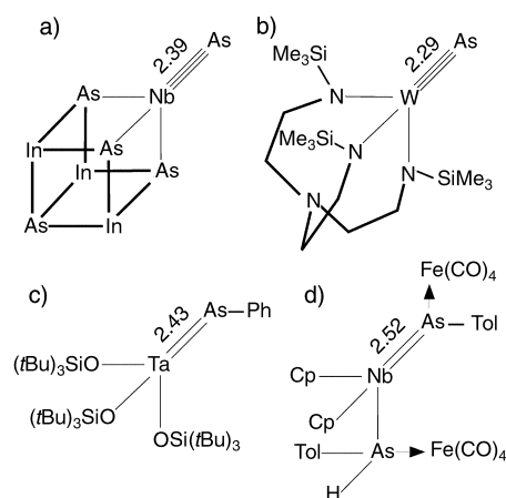
Figure 2. Species with similar coordination around the transition metal: a) [[As(InAs)_3]Nb=As]^{7-} , b) [[N(CH_2CH_2(Me_3Si)N)_3]W\equiv As] ; c) [[tBu_3SiO)_3Ta=As-Ph] , and d) [(Cp)_2(H(Tol))[Fe(CO)_4]As]Nb=As(Tol)-[Fe(CO)_4] .
