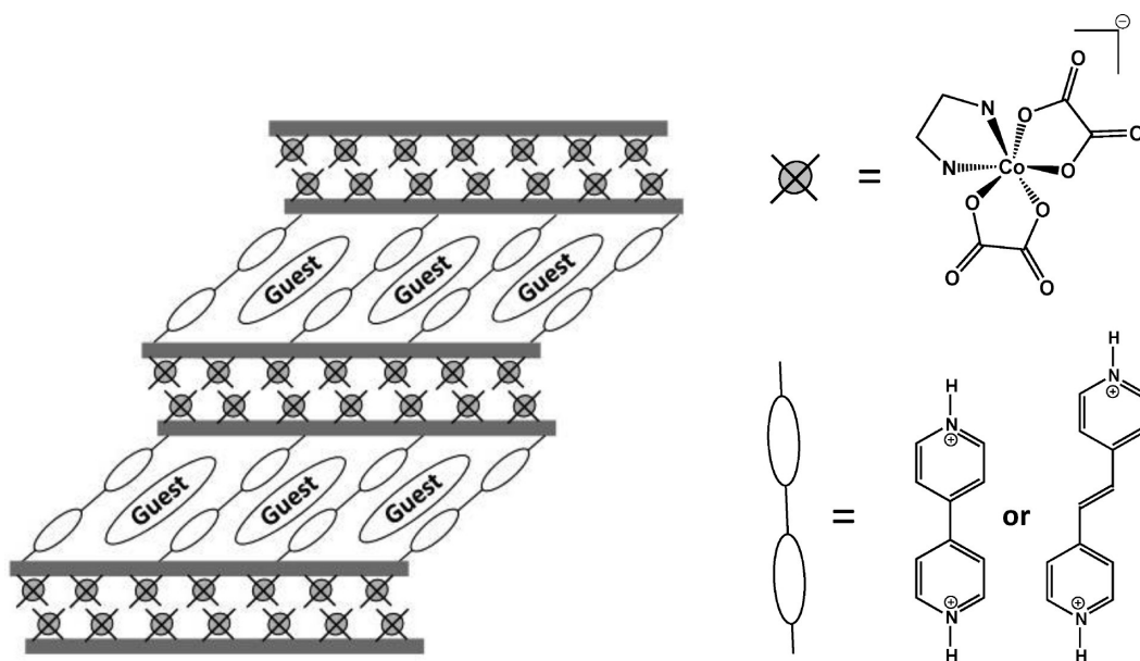
Scheme 1. Schematic Representation of the Typical Pillared-Layer Framework Structures Formed of the Anionic Metal Complex [\text{Co}(\text{en})(\text{ox})_2]^- and the Cationic Bipyridinium Pillars (\text{H}_2\text{bpy})^{2+} and (\text{H}_2\text{bpye})^{2+}
