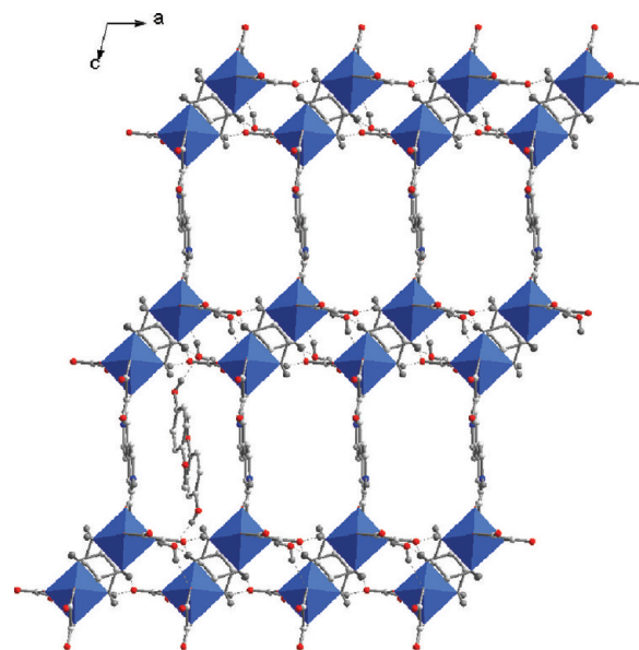
Figure 3. Structure of [H_2bpy][Co(en)(ox)_2]_2 \cdot 2(mp) \cdot H_2O ( 3 ) with 4-methoxyphenol guest molecules (shown in only one gallery).
