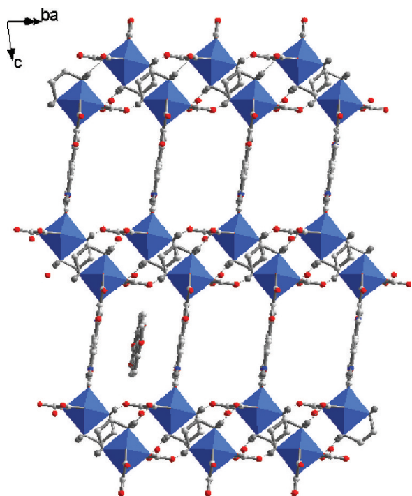
Figure 5. Structure of [\text{H}_2\text{bpy}][\text{Co}(\text{en})(\text{ox})_2]_2 \cdot (\text{dmn}) \cdot \text{H}_2\text{O} (5) with 1,6-dimethoxynaphthalene guest molecules (shown in only one gallery).
