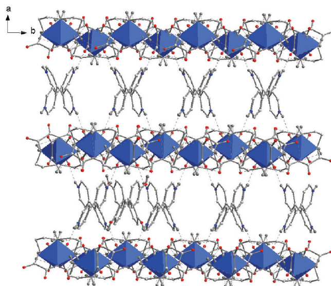
Figure 2. Structure of [H_2bpy][Co(en)(ox)_2]_2 \cdot (bp) \cdot 5H_2O with 4,4'-biphenol guest molecules (shown in only one gallery). The tilt direction of both the pillars and the guests alternates left and right on going along the galleries (the viewing direction).
