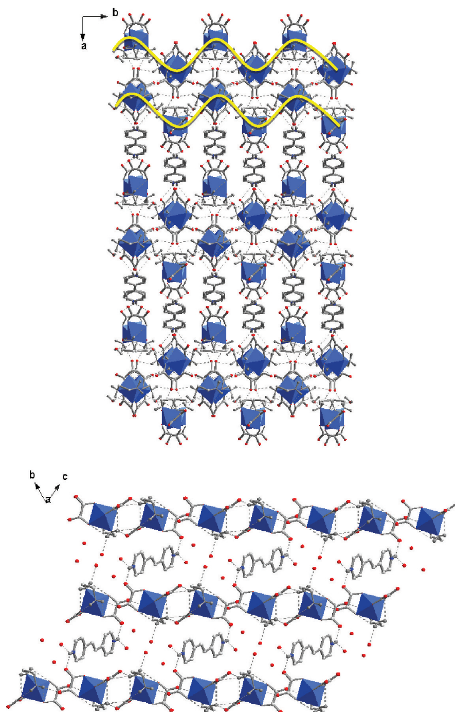
Figure 1. Structures of the guest-free compounds [\text{H}_2\text{bpy}][\text{Co}(\text{en})(\text{ox})_2]_2 \cdot \text{H}_2\text{O} ( 1 , top) and [\text{H}_2\text{bpye}][\text{Co}(\text{en})(\text{ox})_2]_2 \cdot 3\text{H}_2\text{O} ( 6 , bottom). Both are fairly well packed although the extra water in the latter can be viewed as a guest that makes the structure more open. While the metal complexes form flat single layers in 6 , the layers are double and wavy in 1 (outlined in yellow). Hydrogen bonds (broken lines) are found between the complex and the pillars, as well as between the different ligands within the layers.
