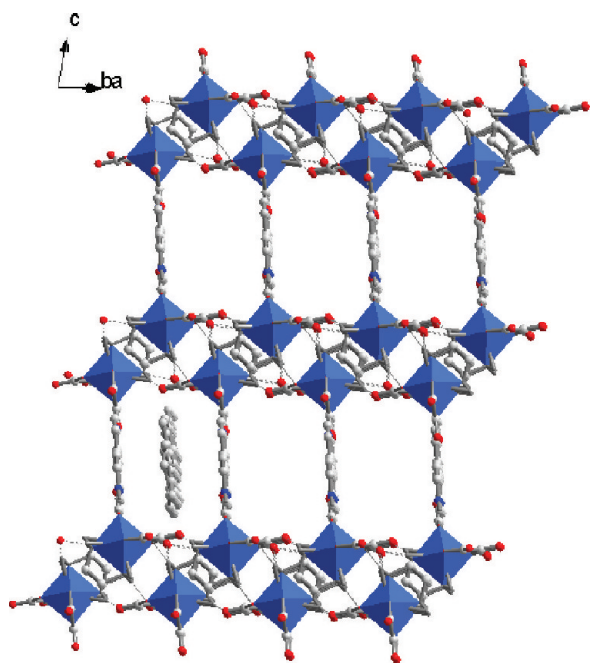
Figure 4. Structure of [\text{H}_2\text{bpy}][\text{Co}(\text{en})(\text{ox})_2]_2 \cdot (\text{dmb}) \cdot \text{H}_2\text{O} (4) with 1,4-dimethoxybenzene guest molecules (shown in only one gallery).
