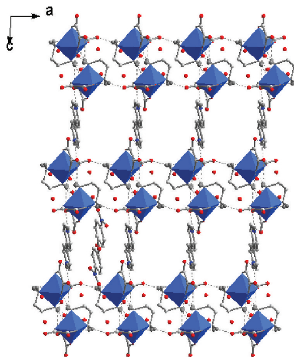
Figure 6. Structure of [\text{H}_2\text{bpye}][\text{Co}(\text{en})(\text{ox})_2]_2 \cdot 2(\text{na}) \cdot 3\text{H}_2\text{O} (7) with 4-nitroanisole guest molecules (shown in only one gallery).
