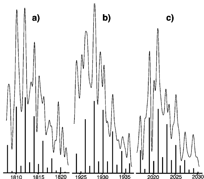
Figure 7. Segments of the electrospray mass spectrum in negative-ion mode of [\text{K}-(18\text{-crown-6})_4\mathbf{3}\cdot 3\text{en}] in DMF: (a) \{(\text{K}^+)([\text{Bi}_6\text{Ni}_6(\text{CO})_6]^{2-})\}^- , (b) \{(\text{K}^+)([\text{Ni}@\text{Bi}_6\text{Ni}_6(\text{CO})_8]^{2-})\}^- , and (c) \{(\text{K}^+\text{-crown})([\text{Bi}_6\text{Ni}_6(\text{CO})_4]^{2-})\}^- .
