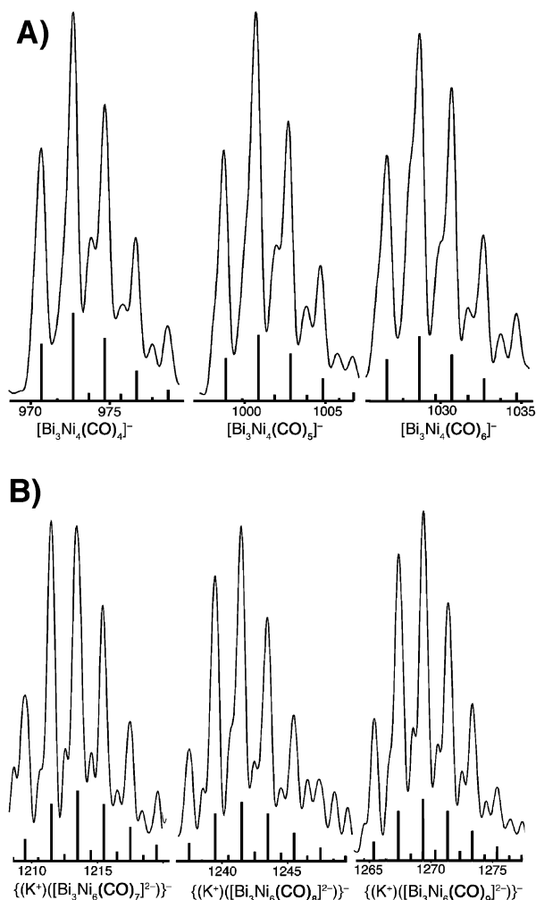
Figure 6. Segments of the electrospray mass-spectra in negative-ion mode of [\text{K}-(2,2,2\text{-crypt})_3\mathbf{1}\cdot\text{en}\cdot\text{tol}] (A) and [\text{K}-(18\text{-crown-6})_3\mathbf{4}\cdot\text{en}\cdot 0.5\text{tol}] (B) dissolved in DMF. The peaks and the theoretical isotope distributions correspond to cluster 1 and cluster 4 (ion-paired with \text{K}^+ ), respectively, and their derivatives missing one and two carbonyl groups. The loss of CO occurs during the electrospray experiment.
