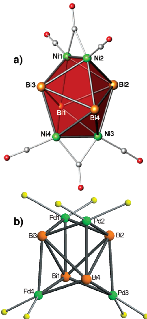
Figure 3. (a) Bisdiphenoidal cluster 2 , [\text{Bi}_4\text{Ni}_4(\text{CO})_6]^{2-} , and (b) [\text{Bi}_4\text{Pd}_4(\text{PPh}_2\text{Me})_8]^{2+} isoelectronic with 2 but with long Pd–Pd distances. 47
