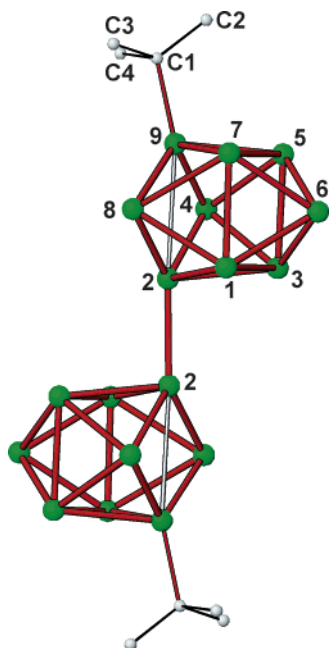
Figure 1. The dialkylated dimer [\text{tBu-Ge}_9\text{-Ge}_9\text{-tBu}]^{4-} with the germanium atoms numbered (the two halves are related by an inversion center). There are two positions for the tBu groups, but only one is shown. Each \text{Ge}_9 cluster is a tricapped trigonal prism (atoms 4, 6, and 8 are capping) with one elongated prismatic edge (shown in white) along which the exo-bonding occurs.
