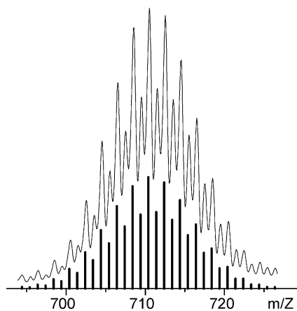
Figure 2. {}^n\text{Bu-Ge}_9^- observed in the ES-MS (negative-ion mode) of a DMF solution of 1 . Shown under the peak is the theoretical isotope distribution for the anion.
