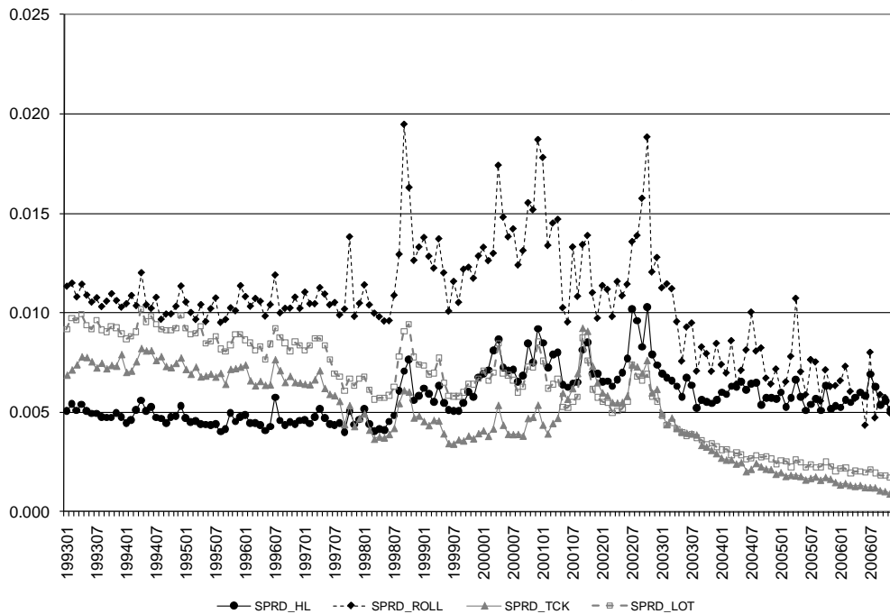
Panel B. Median Absolute Errors by Month
