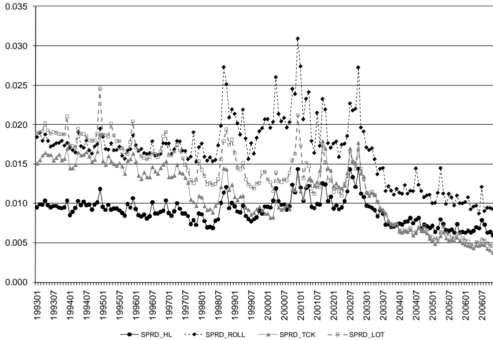
Panel A. Mean Absolute Errors by Month
