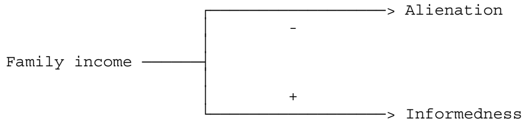
Figure 3. Common cause; Spurious Association
