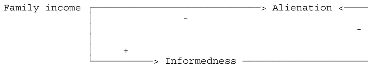
Figure 1. Full Model
