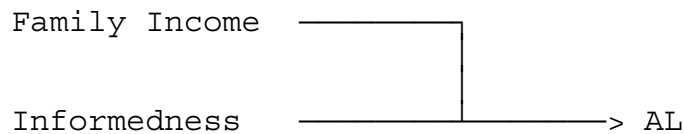
Figure 4. Interaction effects
