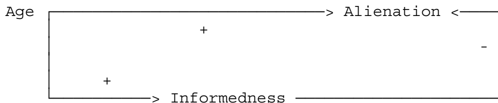
Figure 5. Suppressor effects
