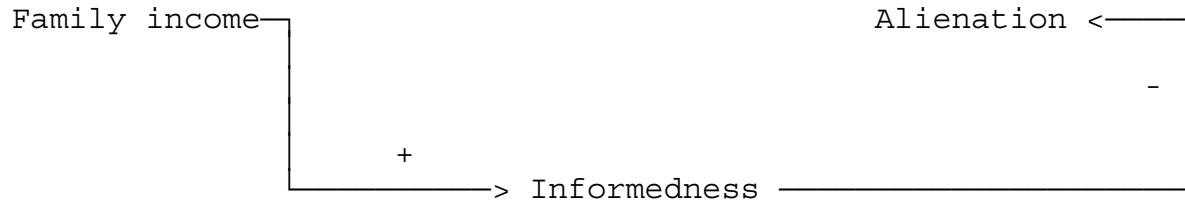
Figure 2. Indirect effects
