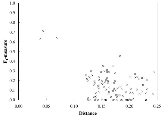
Fig. 4. The correlation between HD-IG distance output and weighted ensemble classification performance. This plot is computed based on the compustat data set.
