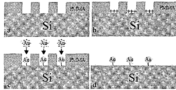
Figure 2. Schematic of Au nanoparticle attachment and liftoff process. a) formation of PMMA trenches by EBL and developed at 6 deg. C; b) sample is soaked in p-lysine for 10 min to make trench bottom positively charged; c) Au-particle attachment for 10-20 hours; d) PMMA removed by acetone or 2-dichlorobenzene [26], leaving the liftoff patterns of Au nanoparticles.
