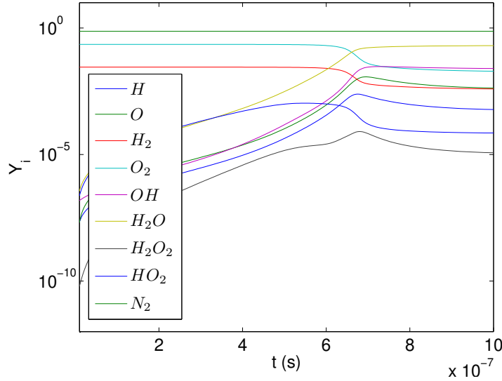
Figure 1.18: Plot near thermal explosion time of Y_{H_2}(t) , Y_H(t) , Y_O(t) , Y_{O_2}(t) , Y_{OH}(t) , Y_{H_2O}(t) , Y_{HO_2}(t) , Y_{H_2O_2}(t) , Y_{N_2}(t) , for adiabatic, isochoric combustion of a mixture of 2H_2 + O_2 + 3.76N_2 initially at T_o = 1542.7 K, P_o = 2.8323 \times 10^6 Pa.
