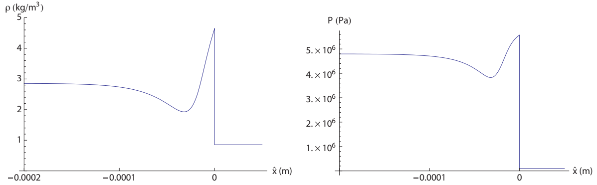
Figure 10.18: ZND structure of \rho(\hat{x}) and P(\hat{x}) for strong D = 2800 m/s > \tilde{D} for two-step irreversible reaction with parameters of Table 10.3.
