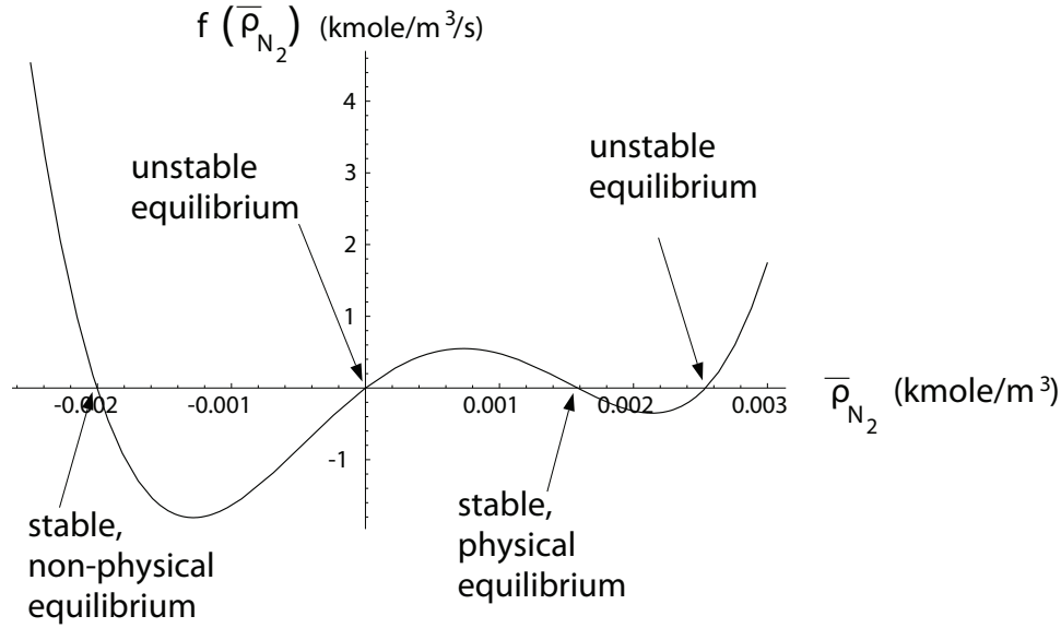
Figure 4.4: Forcing function, f(\bar{p}_{N_2}) , which drives changes of \bar{p}_{N_2} as a function of \bar{p}_{N_2} in isothermal, isobaric problem.
