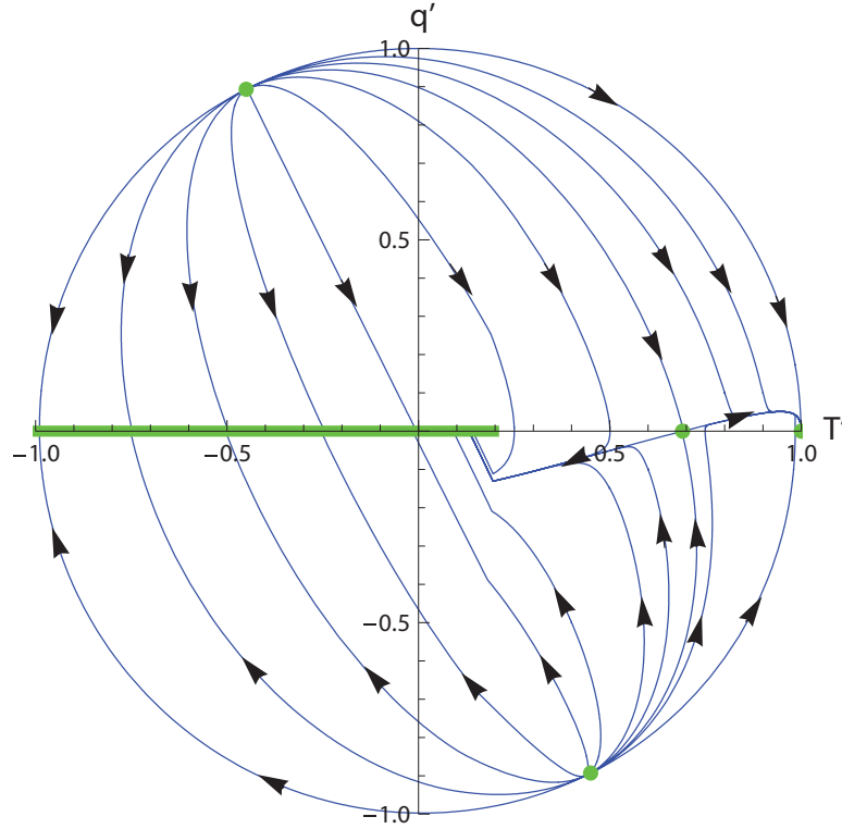
Figure 9.5: Projection of trajectories on Poincaré sphere onto the (T', q') phase plane for a burner-stabilized premixed laminar flame, T_{IG} = 0.2 .
