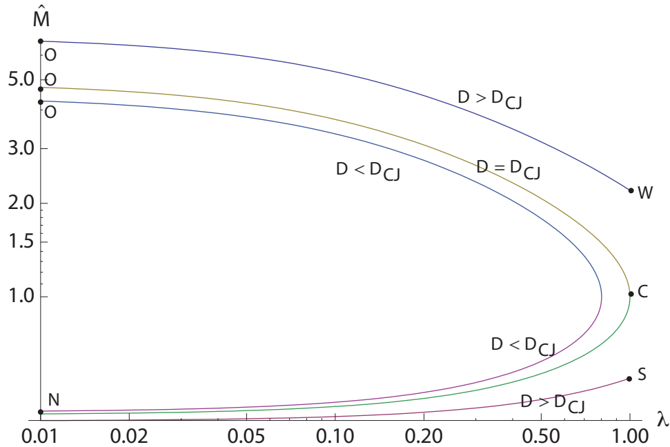
Figure 10.5: \hat{M} versus \lambda from Rankine-Hugoniot analysis for one-step irreversible reaction for D = 2800 m/s > D_{CJ} , D = 1991.1 m/s = D_{CJ} , D = 1800 m/s < D_{CJ} for H_2 /air-based parameters of Table 10.1.
