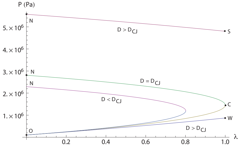
Figure 10.4: P versus \lambda from Rankine-Hugoniot analysis for one-step irreversible reaction for D = 2800 m/s > D_{CJ} , D = 1991.1 m/s = D_{CJ} , D = 1800 m/s < D_{CJ} for H_2 /air-based parameters of Table 10.1.
