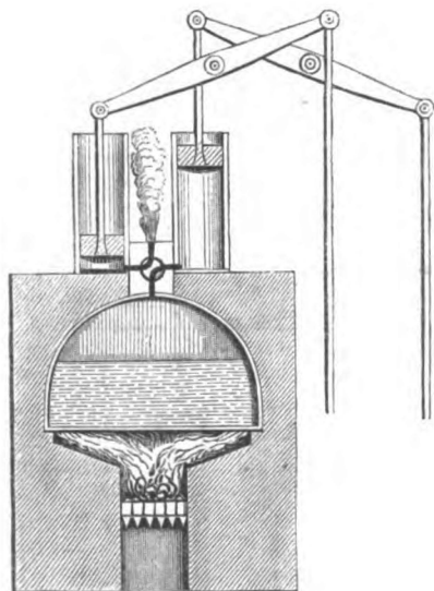
Fig. III.—Leupold's Engine.
