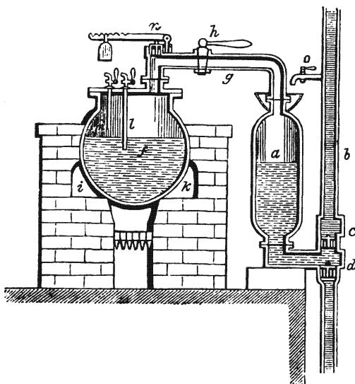
Fig. I.—Savery's Engine.
