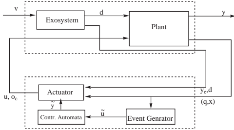
Figure 1: Hybrid systems controller diagram.
