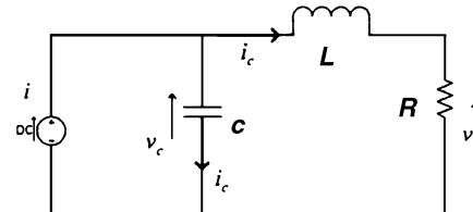
FIGURE 19.1.3 RLC circuit.
