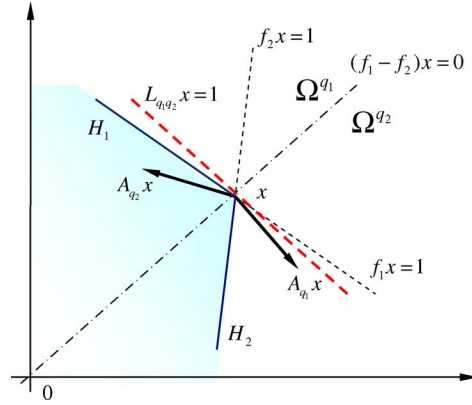
Fig. 3. Case of stable sliding motion.
