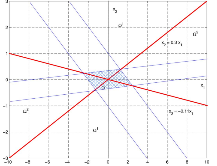
Fig. 7. Intersection of \mathcal{S}_1 and \mathcal{S}_2 and its induced conic partition-based stabilizing switching law.
