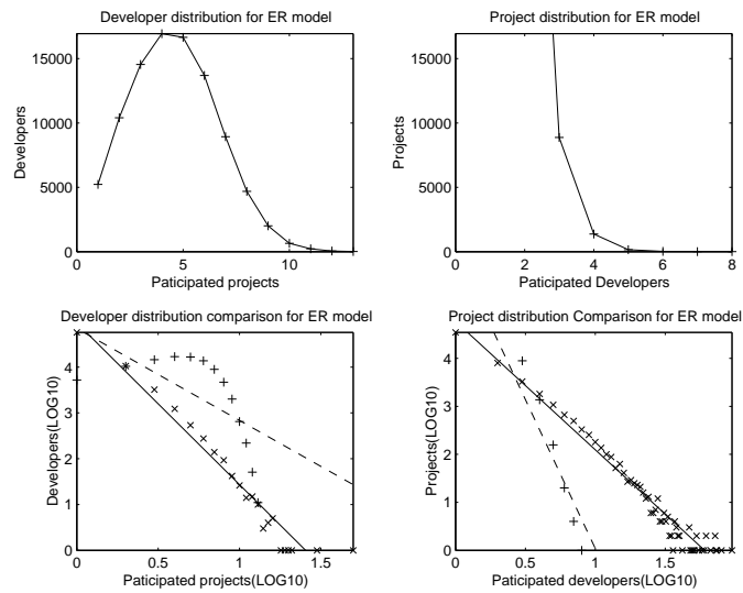
Figure 2: Degree distribution for ER model
