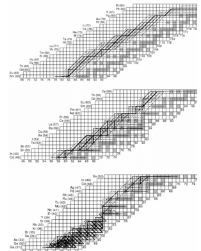
Reaction flow pattern of the p-process. The initial stable seed abundance distribution is converted by (\gamma, n) processes to a distribution of neutron deficient isotopes. This is followed by (\gamma, \alpha) alpha dissociation of the heavy isotopes towards lower masses. Alpha dissociation is hindered at closed shells N=82, Z=50, and N=50 . This flow hindrance is bypassed by alternative \gamma induced neutron or proton dissociation processes. Below N=50 , the alpha binding energy is too high and alpha photo-dissociation disappears.
