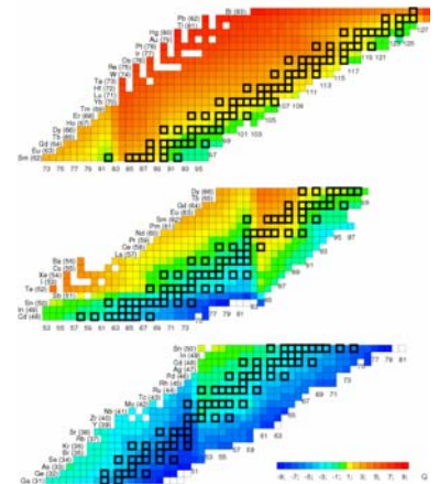
Alpha thresholds in isotopes above Z=30 (Zn). The isotopes marked in yellow to red are alpha unbound and alpha decay easily at high gamma flux conditions by photodisintegration, the green to blue marked isotopes have increasingly higher binding energies and are more difficult to undergo photon induced alpha dissociation. Closed shells are characterized by drastic changes in alpha binding energy.
