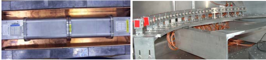
Clover Detector (left) and Si detector (right) arrangements for p-process cross section studies by activation and elastic scattering measurements.
