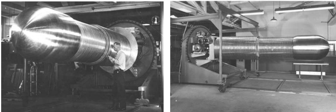
Figure 4. The next generation 4 MV Van De Graaff accelerator built in 1955. The machine was used both with negative charged terminal for the electron beam and with positive charged terminal for charged particle beams for low energy transfer reaction measurements.
