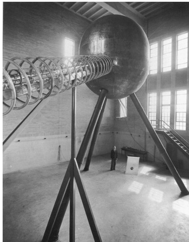
Figure 1. A 1937 photograph of the first Notre Dame accelerator, facing SE. Standing in the background is George Collins. At the time there was one belt, running to the lower left in the picture, The accelerator tube with one corona ring to each drift tube runs towards the upper left.
