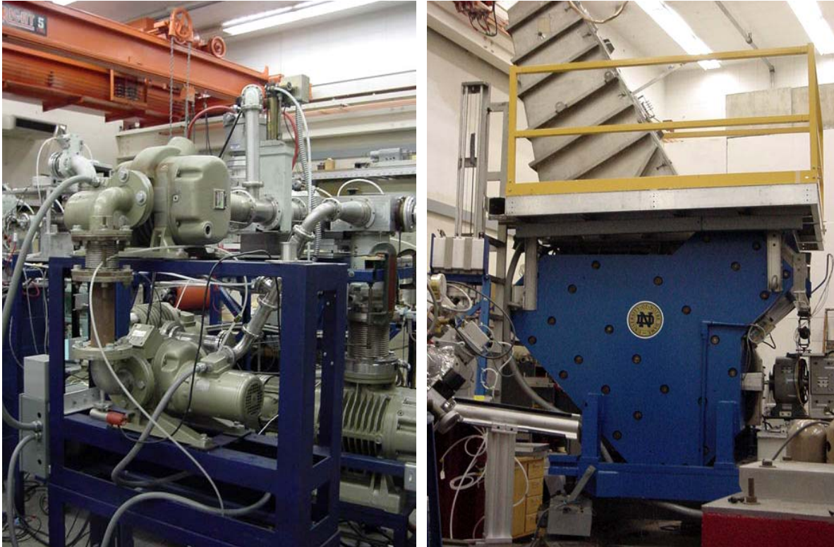
Figure 8. Experimental equipment at the NSL; the left hand side picture shows the windowless gas target systems built from components provided by Ohio State University; the right hand side picture shows the newly painted 100 cm broad range spectrograph which is presently being rebuilt.
