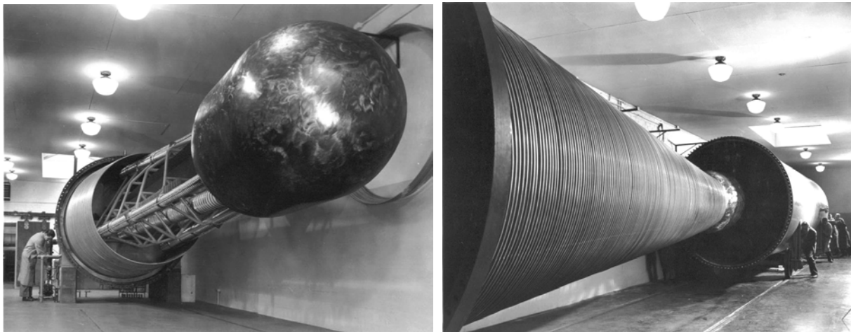
Figure 3. The picture on the left shows the open accelerator column, with the dome still mounted at the terminal while the hubs have been partly removed to allow free access to the column. The picture on the right shows the closing of the rail-guided tank by the technical staff.
