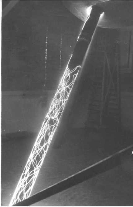
Figure 2. High voltage (~1.2 MV) spark running along one of the 20ft long insulating accelerator legs.
