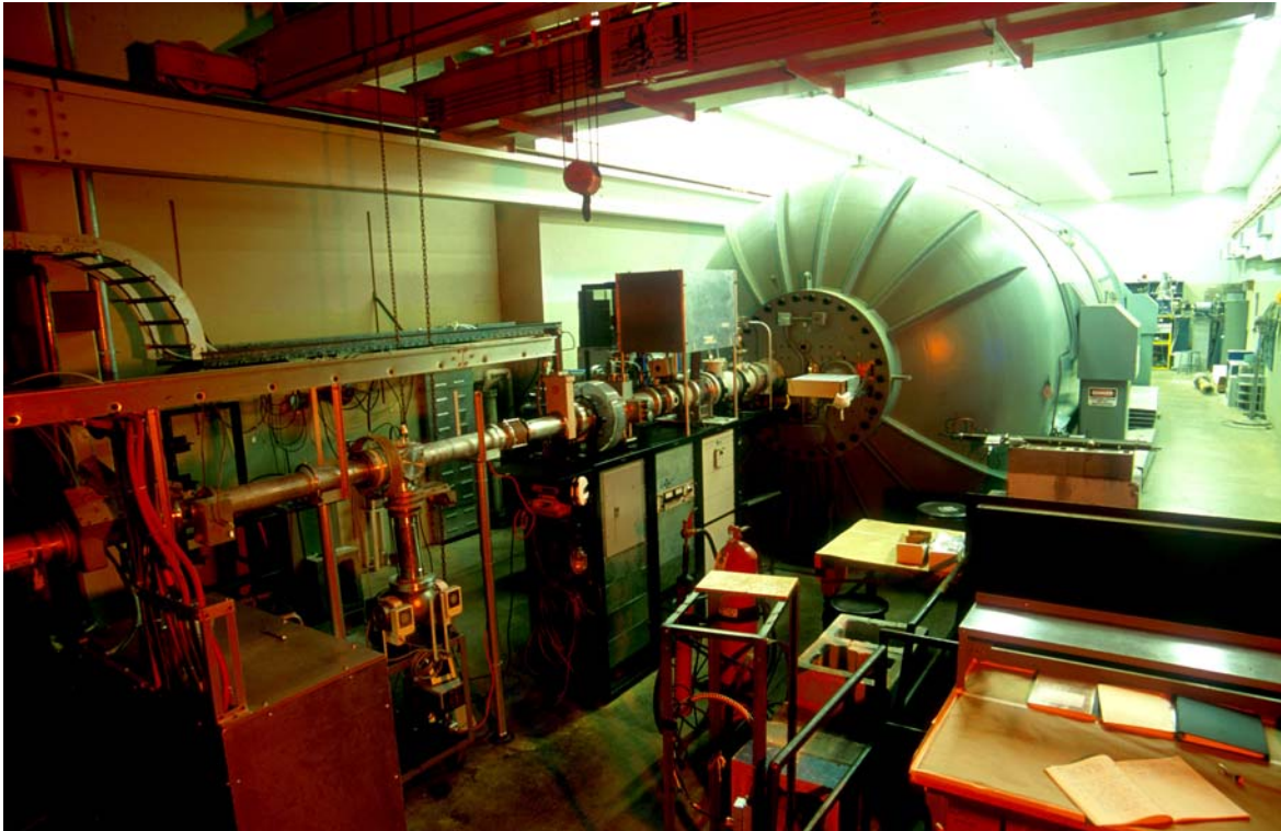
Figure 5. The FN tandem accelerator at the Notre Dame Nuclear Structure Laboratory seen from the low energy side (injector beam line). The tandem is presently operated with a terminal voltage of up to 11 MV. There are two ion sources, a duoplasmatron source which is mainly used for helium beams and a SNICS sputter source for the production of heavy ion beams.
