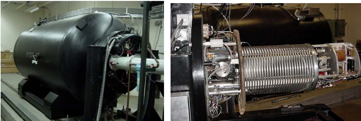
Figure 7. The 3.5 MV KN VdG accelerator is shown at the left hand side, the right hand side shows the short completely rebuilt accelerator column of the 1MV JN VdG, in the background is the tank of the KN machine.
