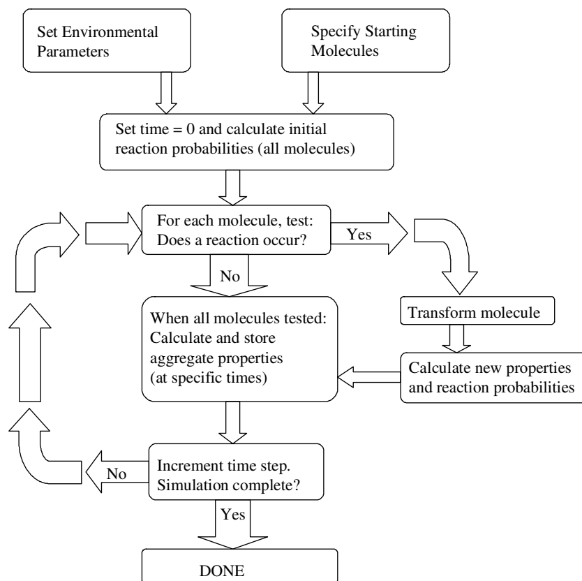
Figure 3. Algorithm outline.
