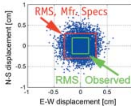
▲ FIGURE 2 Example of static calibration test with manufacturer-predicted RMS bounds and observed bounds from experimental testing
