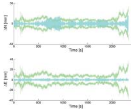
FIGURE 9 Example of Position Quality Thresholds (green) for evaluating reliability of GPS displacements (light blue) of tall building in Chicago on November 30, 2002
