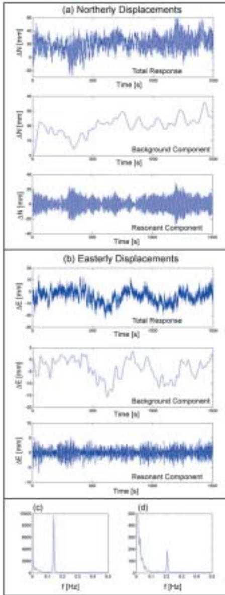
FIGURE 8 Sample of GPS sway displacements of tall building in Chicago under winds on January 7, 2003, decomposed into background and resonant components for (a) Northerly and (b) Easterly displacements with power spectra for GPS displacements along (c) Northerly and (d) Easterly axes of the building
