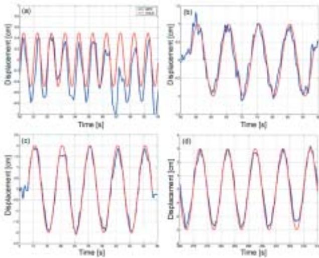
▲ FIGURE 3 Verification of GPS dynamic tracking ability for sine wave at 0.1 Hz with amplitudes of motion from (a) \pm 0.5 cm, (b) \pm 1.0 cm, (c) \pm 2.0 cm and (d) \pm 3.0 cm. GPS displacements blue, shaking table motion red.
