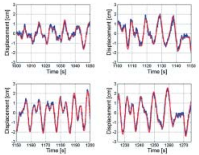
▲ FIGURE 4 Verification of GPS dynamic tracking ability for simulated building response at various times. GPS displacements blue, shaking-table motion red.
