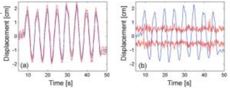
FIGURE 6 Two applications of Position Quality Thresholds for evaluating GPS dynamic displacements: (a) superposition of noise thresholds (red) on tracked displacements (blue); (b) direct threshold plotting (red) for comparison with tracked displacements (blue)
