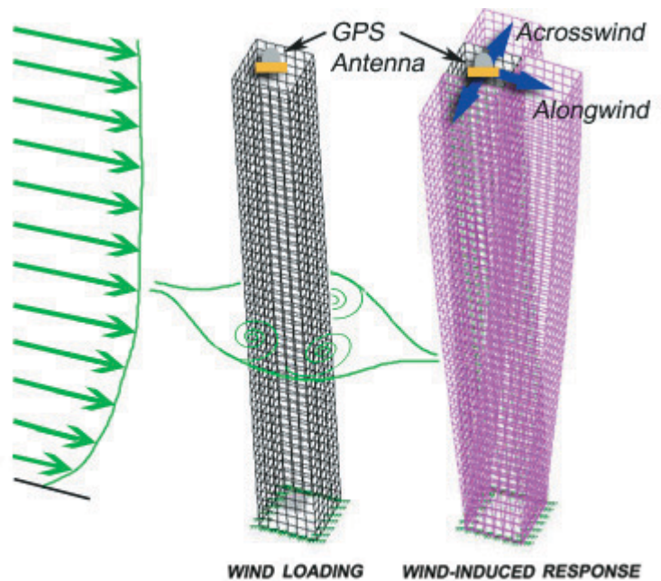
▲ FIGURE 1 Schematic of approaching wind velocity profile impinging on tall building's windward face and separating into vortices impacting the building's other faces (left). This results in the displacement of the building in the direction of the wind (alongwind), as well as side-to-side motions (acrosswind), which can be simultaneously captured by GPS.
