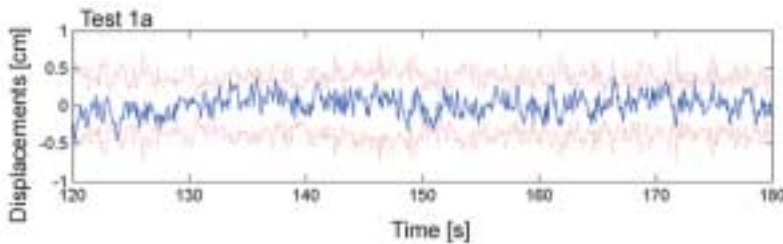
▲ FIGURE 5 Position Quality Threshold validation: constructed noise thresholds (red), compared to background noise in system from three static tests (blue)
