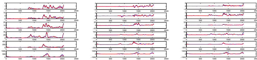
Figure 4: R_{33}(a,t)
