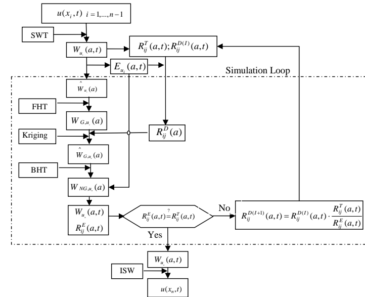
Figure 1: Schematic of the conditional simulation method
