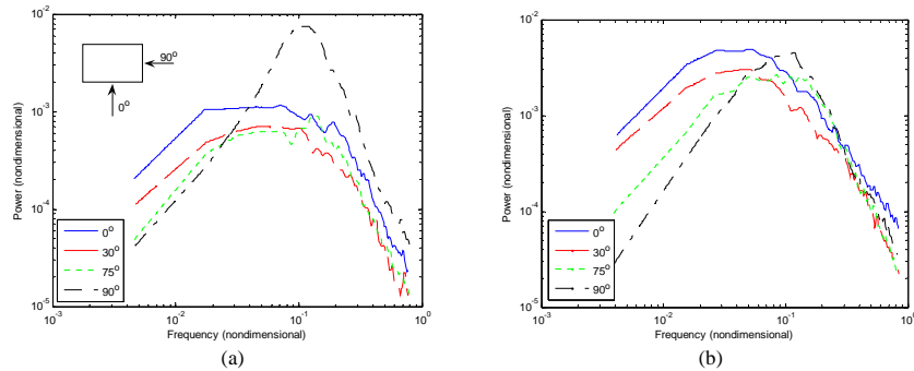
Figure 4: Alongwind loading spectra of the prismatic model at various angles of attack and boundary layer condition (a) BLI and (b) BLII.
