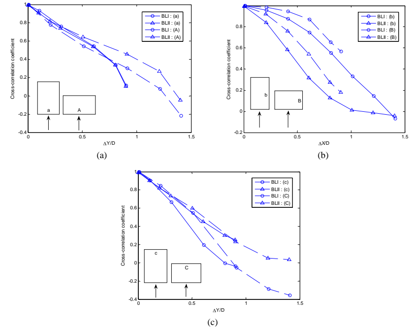
Figure 3: Chordwise cross-correlation structure on the (a) windward, (b) side and (c) leeward surfaces.
