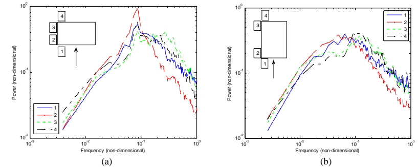
Figure 2: Local spectra of pressure fluctuations in BLII for aspect ratios (a) 0.67 and (b) 1.5
