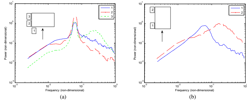
Figure 1: Local spectra of pressure fluctuations in BLI for aspect ratios (a) 0.67 and (b) 1.5
