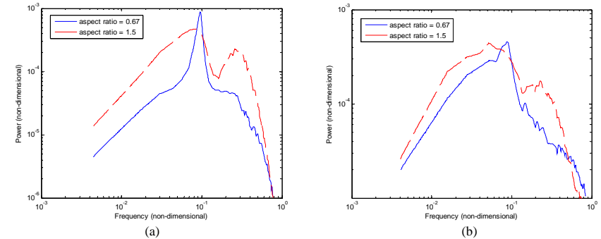
Figure 6: Torsional loading spectra for the prisms within (a) BLI and (b) BLII.
