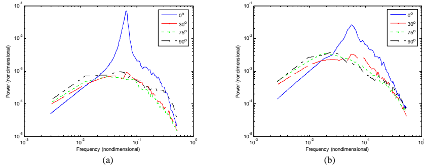
Figure 5: Acrosswind loading spectra of the prismatic model at various angles of attack and boundary layer condition (a) BLI and (b) BLII.
