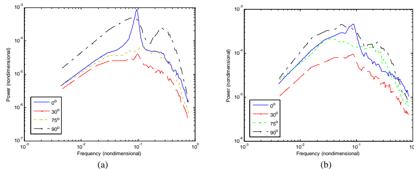
Figure 7: Torsional loading spectra of the prismatic model at various angles of attack and boundary layer condition (a) BLI and (b) BLII.
