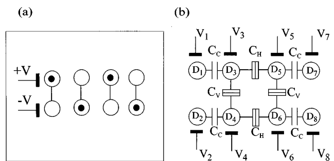
FIG. 1. (a) QCA binary wire. Black dots represent excess electrons. (b) Schematic diagram of experiment. The wire consists of dots D_1 – D_6 . D_7 and D_8 are electrometer dots. External leads and tunnel junctions for the dots and the electrometers are not shown.
