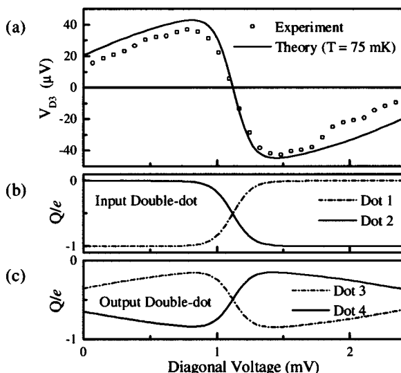
FIG. 5. (a) Experimental and theoretical curves showing the potential change on dot D_3 as a function of the input diagonal voltage. The solid line represents the simulation result at 75 mK, and the dotted line shows the experimental values calculated from the conductance of E_1 . (b) Theoretical calculations of the charges on dots D_1 and D_2 , and (c) dots D_3 and D_4 during QCA polarization change.
