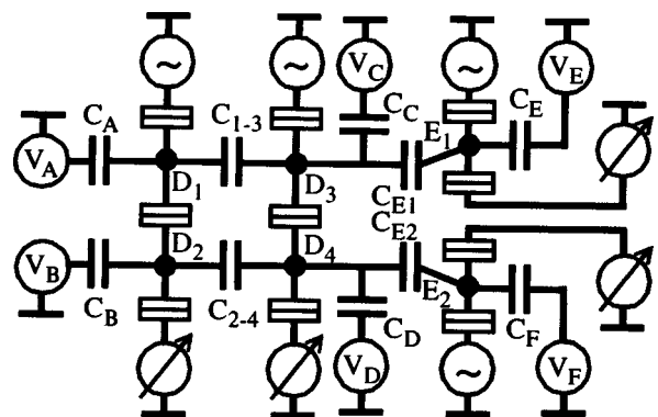
FIG. 1. Schematic diagram of the six-dot system.
