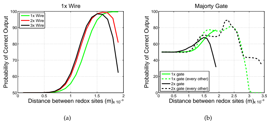
Fig. 7. Probability of a correct output as a function of the distance between redox sites with a DNA scaffolding. (a) considers wires and 0.9 nm between redox sites, (b) considers majority gates using every DNA grid spacing, and every other grid spacing in the y-dimension.
