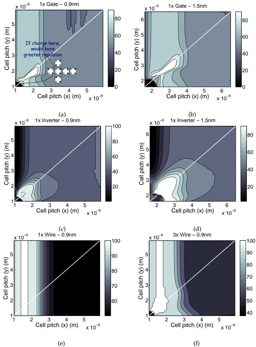
Fig. 3. Probability of a correct logical output as a function of cell spacing. Graphs (a), (c), and (e) look at majority gates, inverters, and wires (all 1 cell thick) with 0.9 nm between redox centers. Graphs (b) and (d) look at majority gates and inverters for a larger molecule (1.5 nm between redox sites). Graph (f) looks at a wire segment 3 cells thick with 0.9 nm between redox sites.
