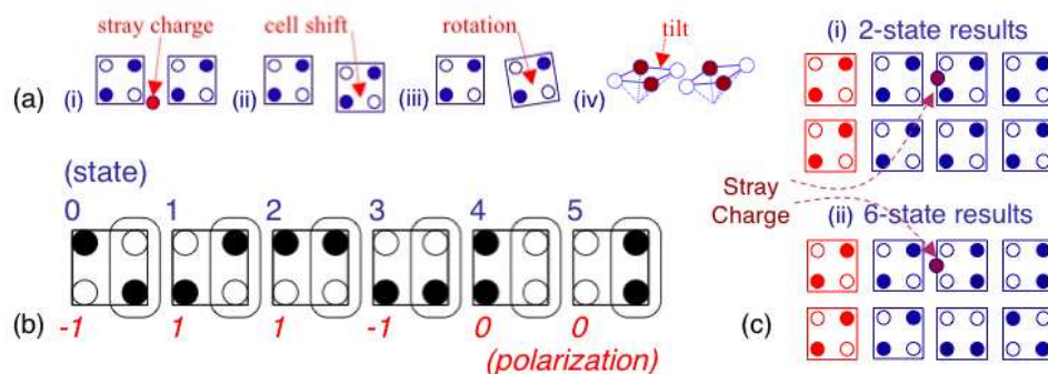
Fig. 2. (a) Expected defects, (b) Possible states of a QCA molecule and “seen” polarizations, (c) Defects may cause degenerate states.
