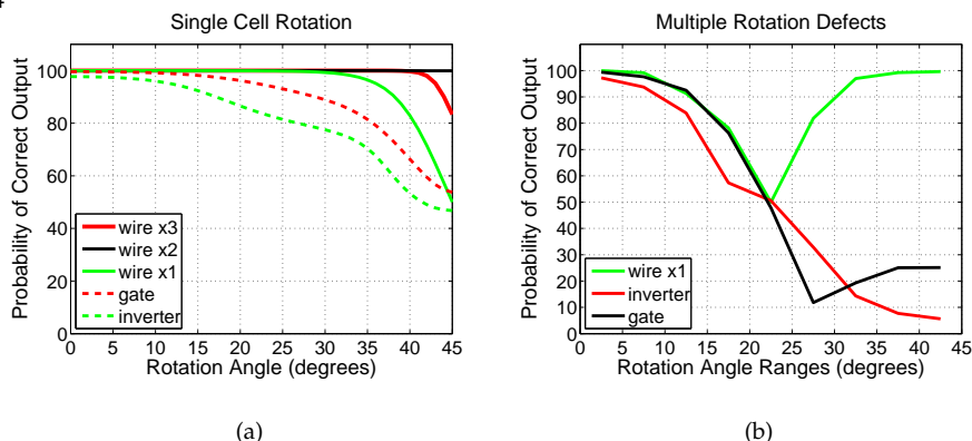
Fig. 6. (a) Effects of rotating one cell, (b) Effects of rotating all cells.
