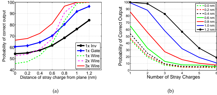
Fig. 5. (a) Effects of a single stray charge, (b) Effects of multiple charges.
