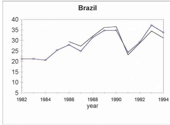
Figure 3: Fit of Spending Model by Country and Year (Black lines are actual spending. Blue lines with circles are model predictions.)
