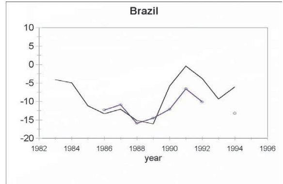
Figure 4: Fit of Fiscal Balance Model by Country and Year (Black lines are actual surpluses or deficits. Blue lines with circles are model predictions.)
