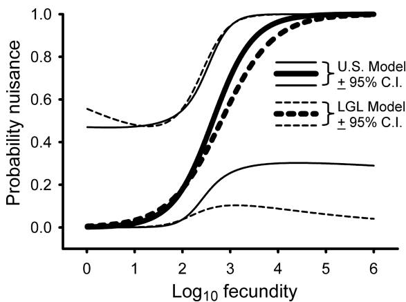
Figure 2. Logistic curves ( \pm 95\% CI) showing the relationship between fecundity and probability of becoming nuisance (i.e., causing economic and/or environmental harm) for molluscs in the Laurentian Great Lakes (LGL) and 48 contiguous states of the United States. For the Great Lakes analysis eight predictor variables were used; fecundity was the only significant one. For the U.S. analysis, fecundity was the only variable used. Fecundity is the annual number of eggs or live offspring released per female.
