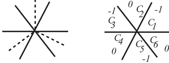
FIGURE 5. The chambers at the vertex of a three-armed star
