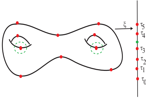
FIGURE 1. The height function on a genus two surface.
