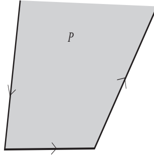
FIGURE 6. A polyhedron in \mathbb{R}^2 and its boundary.
