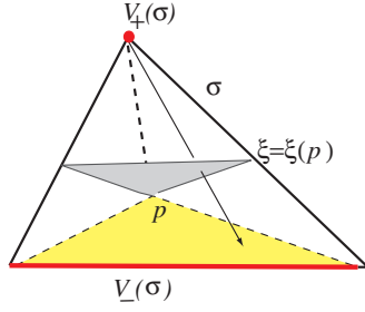
FIGURE 3. The local homotopic structure of critical sublevel sets.
