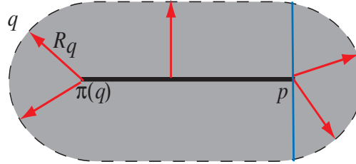
FIGURE 4. The "aura" of a straight line segment in the plane
