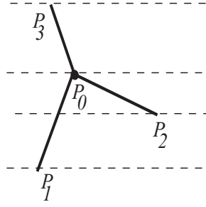
FIGURE 2. A planar star.
