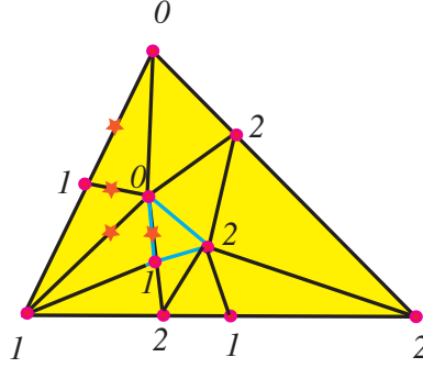
FIGURE 3. A triangulation of a triangle.
