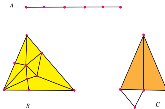
FIGURE 1. Triangulated spaces.
