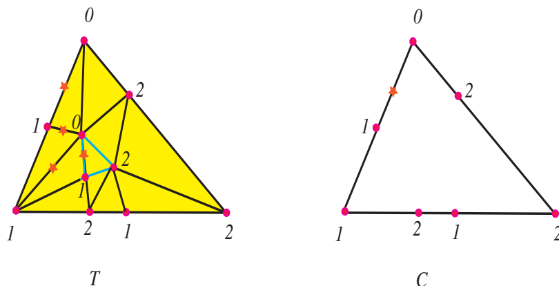
FIGURE 4. A triangulation of a triangle, and the induced triangulation on the boundary.
