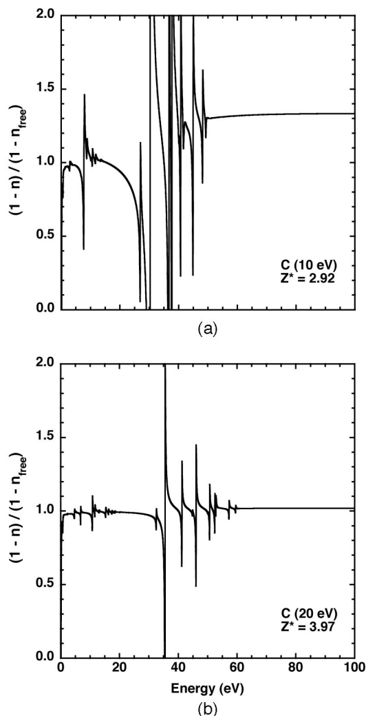
Fig. 5. Ratio (1 - n)/(1 - n_{\text{free}}) versus photon energy for C plasmas with temperatures of (a) 10 and (b) 20 eV. The corresponding ionization Z^* = 2.92 and 3.97, respectively. The ion density is 10^{20} \text{ cm}^{-3} .
