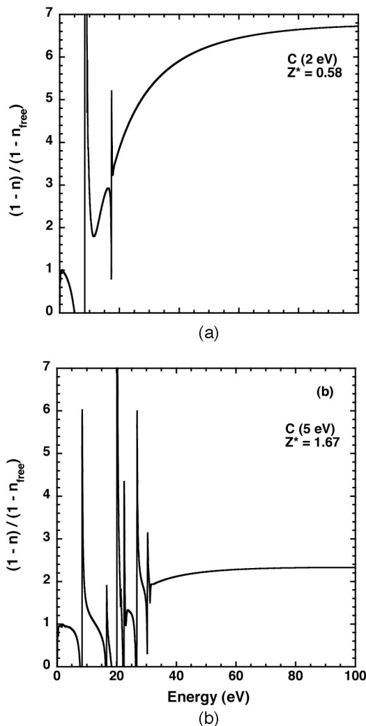
Fig. 4. Ratio (1 - n)/(1 - n_{\text{free}}) versus photon energy for C plasmas with temperatures of (a) 2 and 5 eV. The corresponding ionization Z^* = 0.58 and 1.67, respectively. The ion density is 10^{20} \text{ cm}^{-3} .
