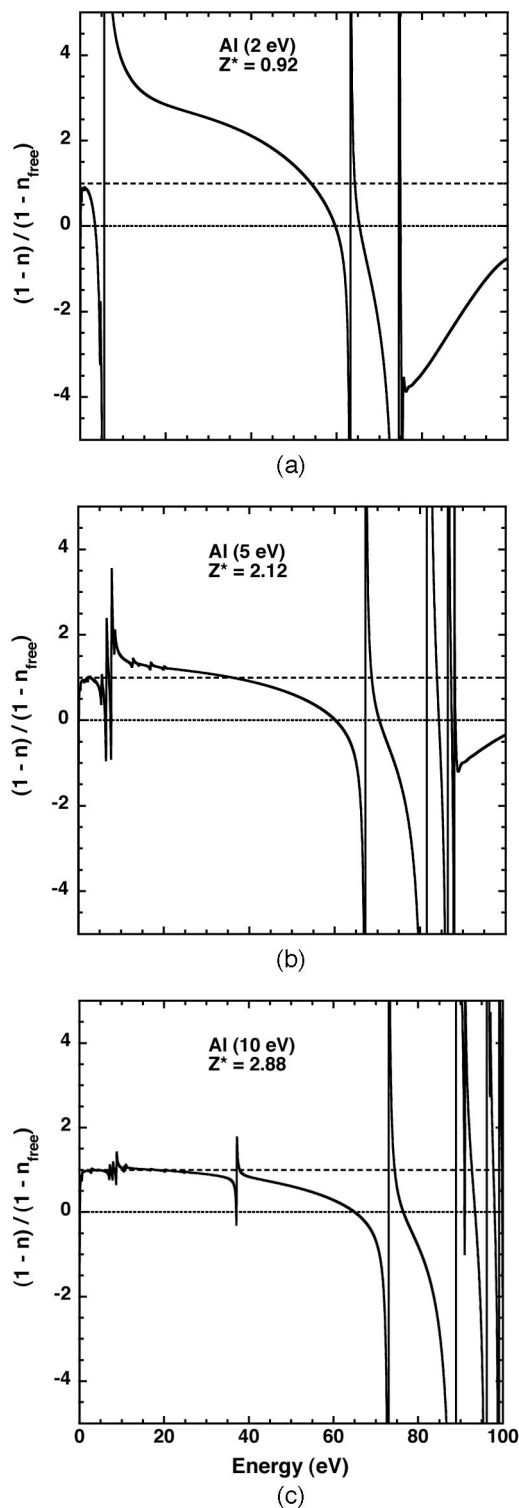
Fig. 1. Ratio (1 - n)/(1 - n_{\text{free}}) versus photon energy for Al plasmas with temperatures of (a) 2, (b) 5, and (c) 10 eV. The corresponding ionization is Z^* = 0.92 , 2.12 and 2.88, respectively. The ion density is 10^{20} \text{ cm}^{-3} . The dotted lines at ratios of 0 and 1 are visual aids.
