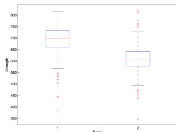
Ceramic Strength by Batch Order
