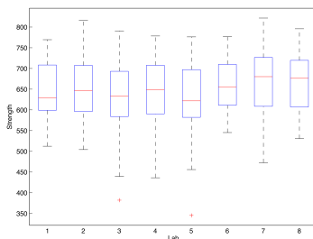
Ceramic Strength by Lab
