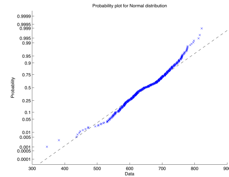
Normal Probability Plot of Ceramics Data from MatLab
