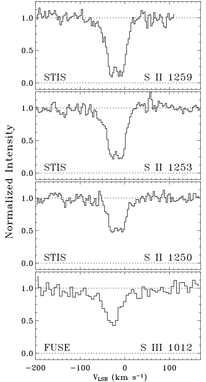
FIG. 2.—Absorption-line profiles of S II \lambda\lambda 1250.584 , 1253.811 , and 1259.519 from STIS E140M observations and S III \lambda 1012.495 from FUSE (see Paper I). We suggested in Paper I that the material at v_{\text{LSR}} \approx -30 \text{ km s}^{-1} was likely associated with the Galactic thick disk given the higher degree of ionization compared with the material at v_{\text{LSR}} \approx -4 \text{ km s}^{-1} . The STIS data have a resolution of \sim 6.5 \text{ km s}^{-1} , while the FUSE data have a resolution of \sim 20 \text{ km s}^{-1} .
