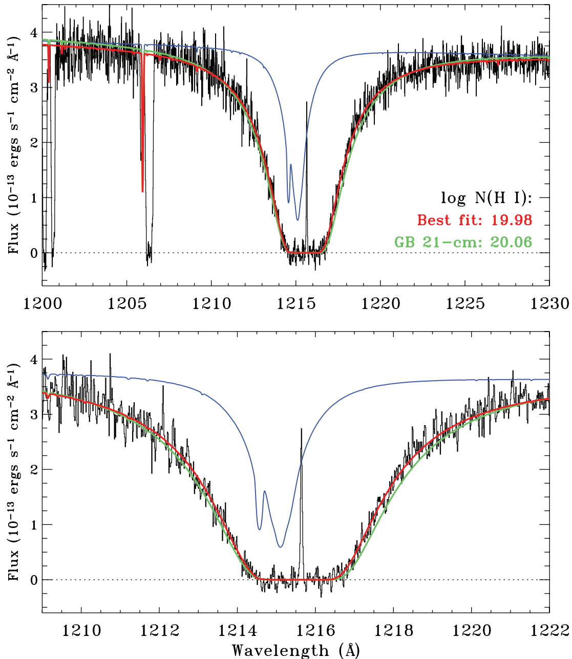
FIG. 1.—Two views of the STIS E140M spectrum of the Ly \alpha absorption profile toward vZ 1128. Both stellar and interstellar absorption contribute to this profile. The estimated stellar profile is shown as the thin blue line and has been shifted to v_{\text{LSR}} = -145 \text{ km s}^{-1} to match the observed positions of stellar absorption lines in the STIS spectrum. The best fit to the interstellar and stellar absorption profile is shown in red, corresponding to an interstellar column density \log N(\text{H I}) = 19.98 \pm 0.03 . The green line shows the best-fit profile adopting the H I column density derived from Green Bank 140 foot telescope observations of 21 cm emission in this direction, \log N(\text{H I}) = 20.04 \pm 0.01 (see Paper I). The sharp emission line in the center of the Ly \alpha absorption trough is geocoronal emission. The strong stellar line near 1206 Å is stellar Si III.
