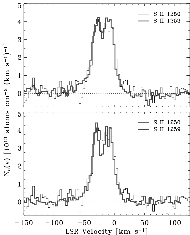
FIG. 3.—Comparison of the apparent column density profiles for S II \lambda\lambda 1250.584, 1253.811, and 1259.519 from STIS E140M observations. The weaker two lines (at 1250.584 and 1253.811 Å) are compared in the top panel; the strongest line (1259.519 Å) is compared with the weakest in the bottom panel. The lack of agreement between these profiles indicates that the stronger line contains a small amount of unresolved saturated structure.
