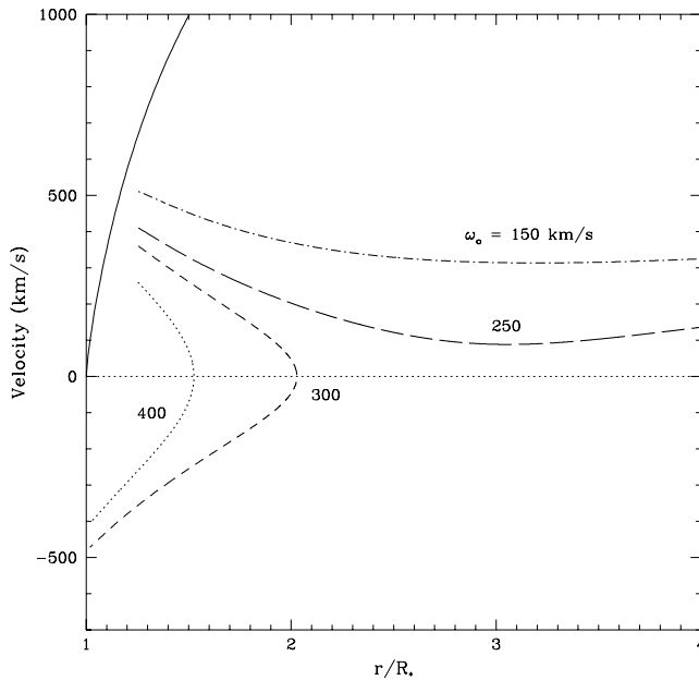
FIG. 4.—Same as Fig. 2, but for clumps of constant mass and initial radii [(\log m_c, r_0) = (19.0, 1.25R_*)] with varying initial relative velocities ( \omega_0 = 150, 250, 300, and 400 \text{ km s}^{-1} ). At this position in the wind, \frac{1}{2}v_w = 331 \text{ km s}^{-1} . The initial relative velocities are labeled for each trajectory.
