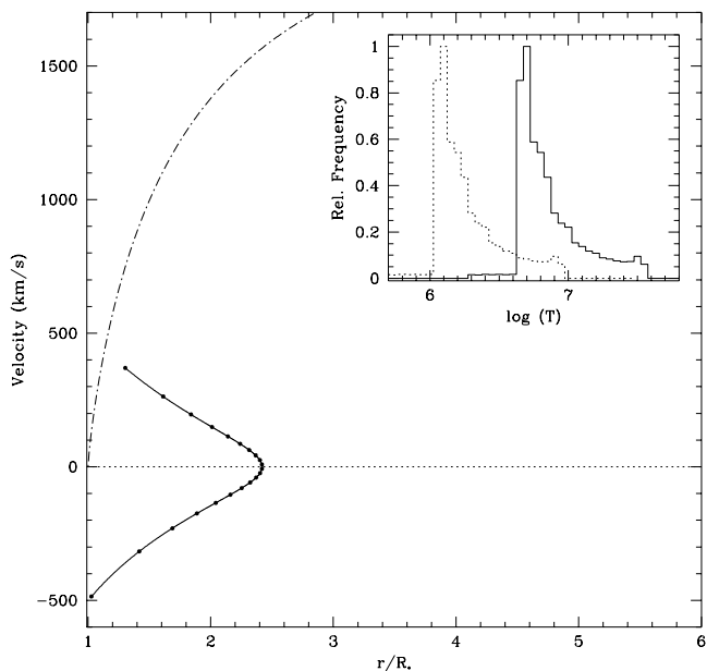
FIG. 5.—Main plot shows a trajectory for a clump with the initial conditions (\log m_c, r_0, \omega_0) = (19.0, 1.30R_*, 371 \text{ km s}^{-1}) . This clump follows an infall trajectory. The trajectory is marked with a dot every 1.25 hr. Also shown is the wind velocity calculated with a \beta velocity law (dot-dashed line). The inset shows the relative distribution of temperatures in the shock-heated gas formed as the clump follows this trajectory. This distribution is weighted by \rho_w(r)^2 for each point along the trajectory to roughly account for the dependence of the X-ray emission on density. The shock-jump velocities, \Delta v , are calculated from the relative velocity between wind and the clump, \omega , such that \Delta v = \omega \cos \theta . The solid distribution of temperatures assumes \theta = 0^\circ , while the dotted distribution uses \theta = 30^\circ .
