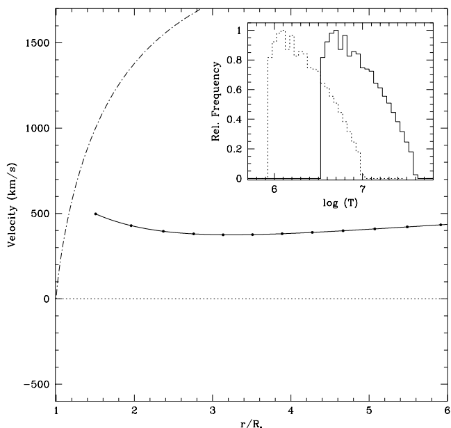
FIG. 6.—Same as for Fig. 5, but for the initial conditions (\log m_c, r_0, \omega_0) = (19.0, 1.50R_*, 498 \text{ km s}^{-1}) . This clump follows an outflow trajectory.
