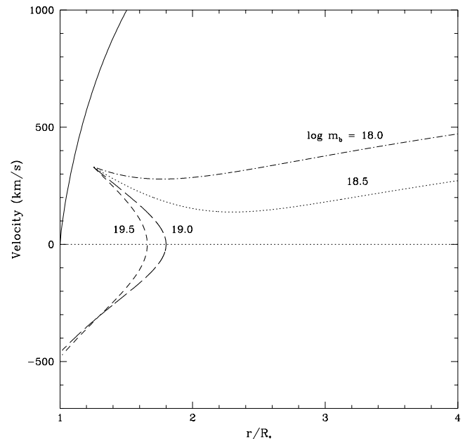
FIG. 2.—Trajectories of clumps forming in the wind of \tau Sco having different initial conditions. The velocity scale is relative to the surface of the star, and the distance from the stellar surface is given in units of stellar radii. Also shown is the \beta velocity law of the ambient stellar wind (solid line). The starting distance from the star and velocity relative to the ambient wind for these clumps are (r_0, \omega_0) = (1.25R_*, 331 \text{ km s}^{-1}) . The four different trajectories represent clumps formed with masses \log m_c = 18.0, 18.5, 19.0 , and 19.5 ( m_c in grams). The masses are labeled for each trajectory. Note the low-mass clumps are pushed outward through the wind, following outflow trajectories. The higher mass clumps are able to fall back onto the star and follow infall trajectories.
