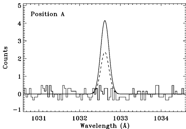
FIG. 2.— FUSE spectrum of the wavelength region around 1032 Å in position A. The observed spectrum (histogram) is binned to 0.037 Å pixel -1 , and a constant background was subtracted. No O VI emission is visible in the spectrum. The smooth lines show the expected number of counts if the O VI emission were equal to the observed 0.3–2.0 keV X-ray flux, after accounting for extinction using the Galactic extinction law (Cardelli et al. 1989; solid line), and the LMC extinction law (Howarth 1983; dashed line). The FWHM of the emission line is assumed to be 0.34 Å ( 100 km s -1 ).
