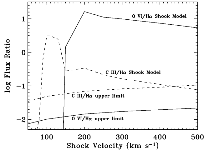
FIG. 3.—Shock model predictions of O VI/H \alpha (solid line) and C III/H \alpha (dashed line) from the models of Dopita & Sutherland (1996; v_s \geq 150 \text{ km s}^{-1} ) and Shull & McKee (1979; v_s < 150 \text{ km s}^{-1} ). The nearly diagonal lines show the observed upper limits at position A, the most restrictive limit of the four pointings. The upper limits are calculated for a line width (FWHM) corresponding to the shock velocity (assuming that bulk motion, not thermal broadening, is responsible for the line width). The upper limits are well below the predictions, indicating that most of the H \alpha -emitting gas is not shock heated, unless the shocks have v_s \leq 90 \text{ km s}^{-1} .
