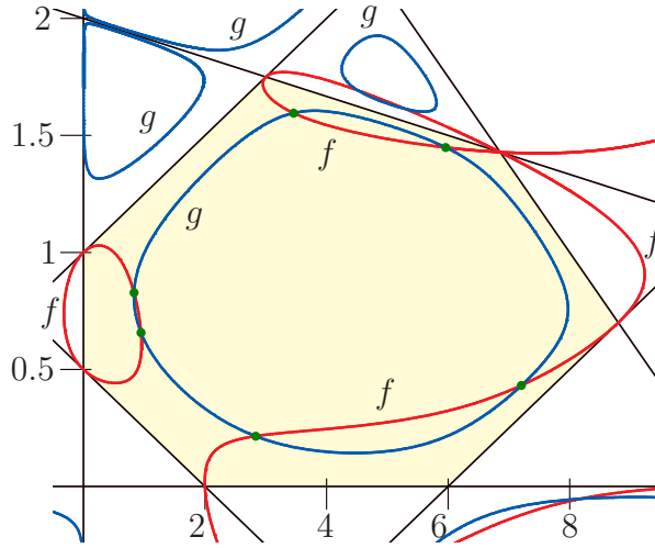
FIGURE 3. Master function curves in the septagon
