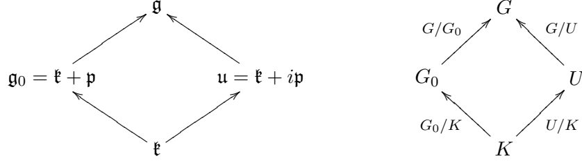
Figure 1: Algebras, groups, and quotients.
