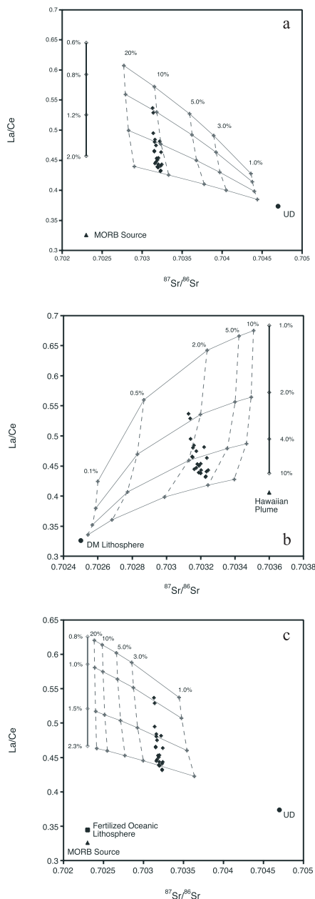
Figure 14. Plots of ^{87}\text{Sr}/^{86}\text{Sr}_I versus La/Ce. (a) Model 1: UD is undepleted mantle (composition is given in Table 6). Curved horizontal lines are mixing lines between incipient melts of MORB source and UD, while vertical lines are lines of equal mixing proportions. (b) Model 2: Mixing of incipient melts of Hawaiian plume (composition given in Table 6) with depleted mantle (DM) lithosphere. Notice that the trend of the data crosscuts the lines of equal mixing proportions. (c) Model 3: Mixing of incipient melts of MORB source refertilized at time of formation by small-degree melts at the mid-ocean ridge with UD. The degree of partial melting is more realistic than the extremely small degrees of melting required by Model 1.
