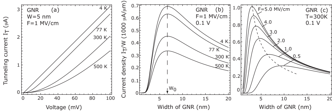
FIG. 2. Tunneling currents in GNR p - n junctions: (a) W=5 nm device, voltage dependence at various temperatures. Tunneling currents per unit width for different GNR widths at (b) various temperatures at \mathcal{F}=1 MV/cm and (c) for various \mathcal{F} at 300 K. To maximize the tunneling current density, an optimum (\mathcal{F}, W) combination exists as illustrated by the dashed lines.
