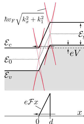
FIG. 1. (Color online) Interband tunneling in a reverse-biased GNR/CNT p - n junction and the potential barrier seen by tunneling electrons.
