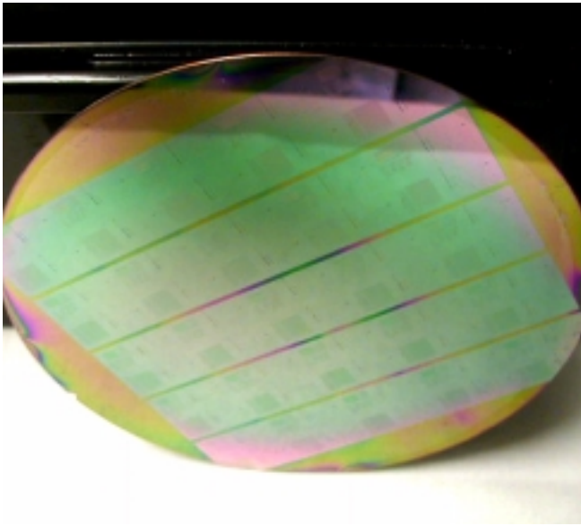
5 Min. Purple at edges Purple means thin polysilicon
