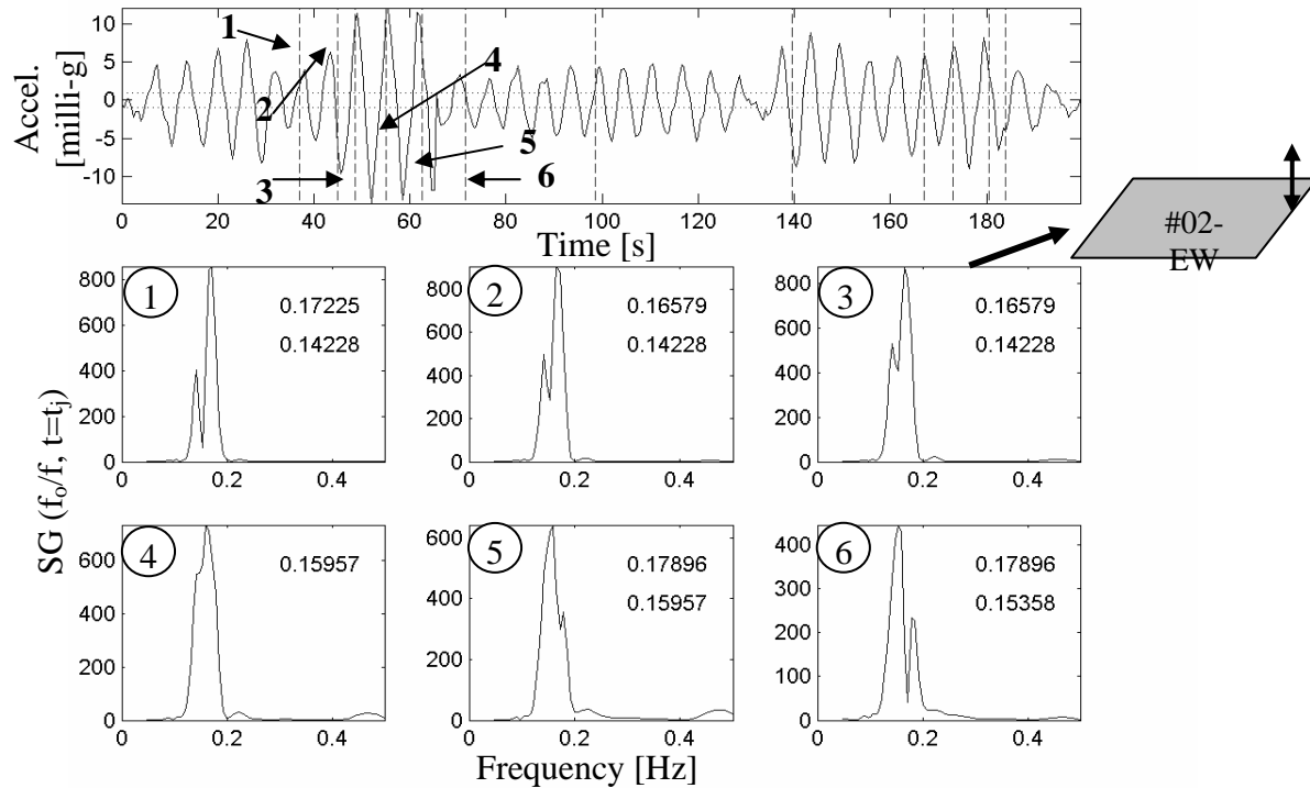
Figure 5. Acceleration response at #02-EW with wavelet instantaneous spectral analysis for March 10, 1974.
