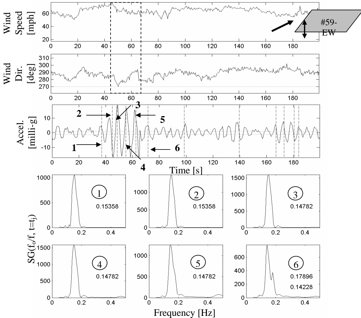
Figure 4. Wind speed, direction and acceleration at #59-EW with wavelet instantaneous spectral analysis for March 10, 1974.
