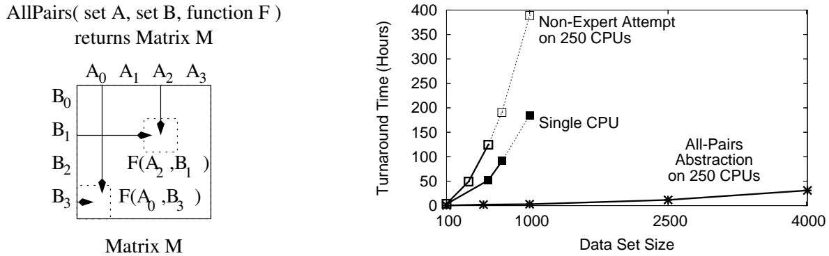
Fig. 1. The All-Pairs Problem
